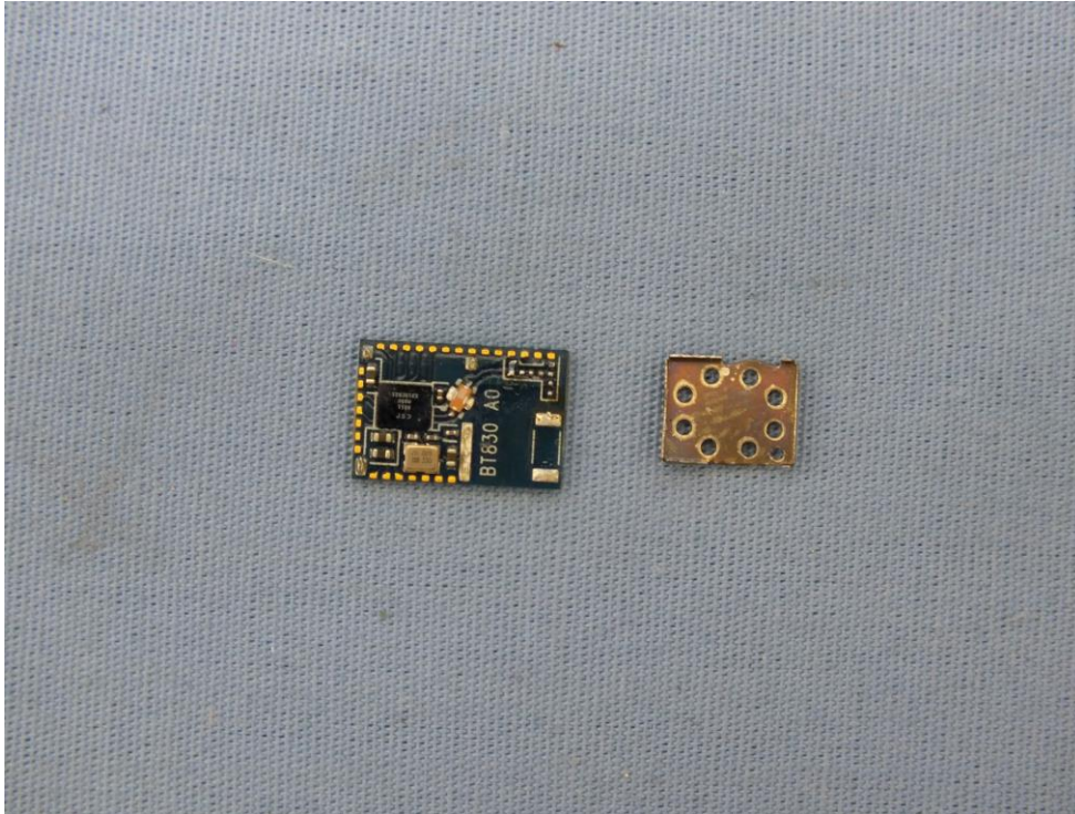
Model: BT830-ST
