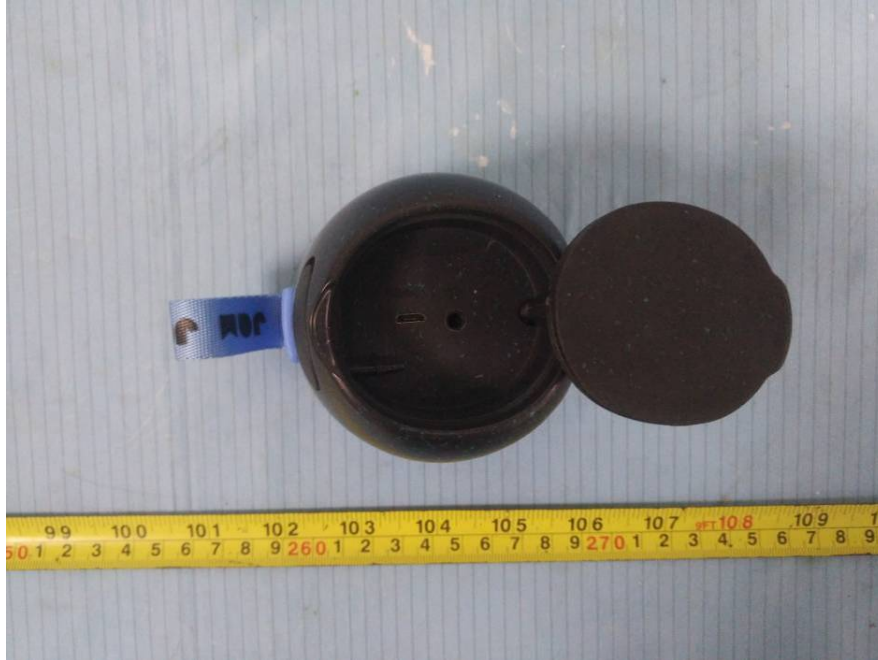
EUT – Charging Port & Audio Port View
