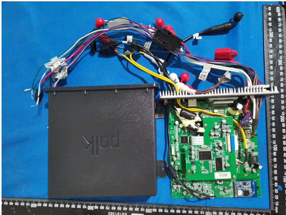
Tuner/Amp Module
