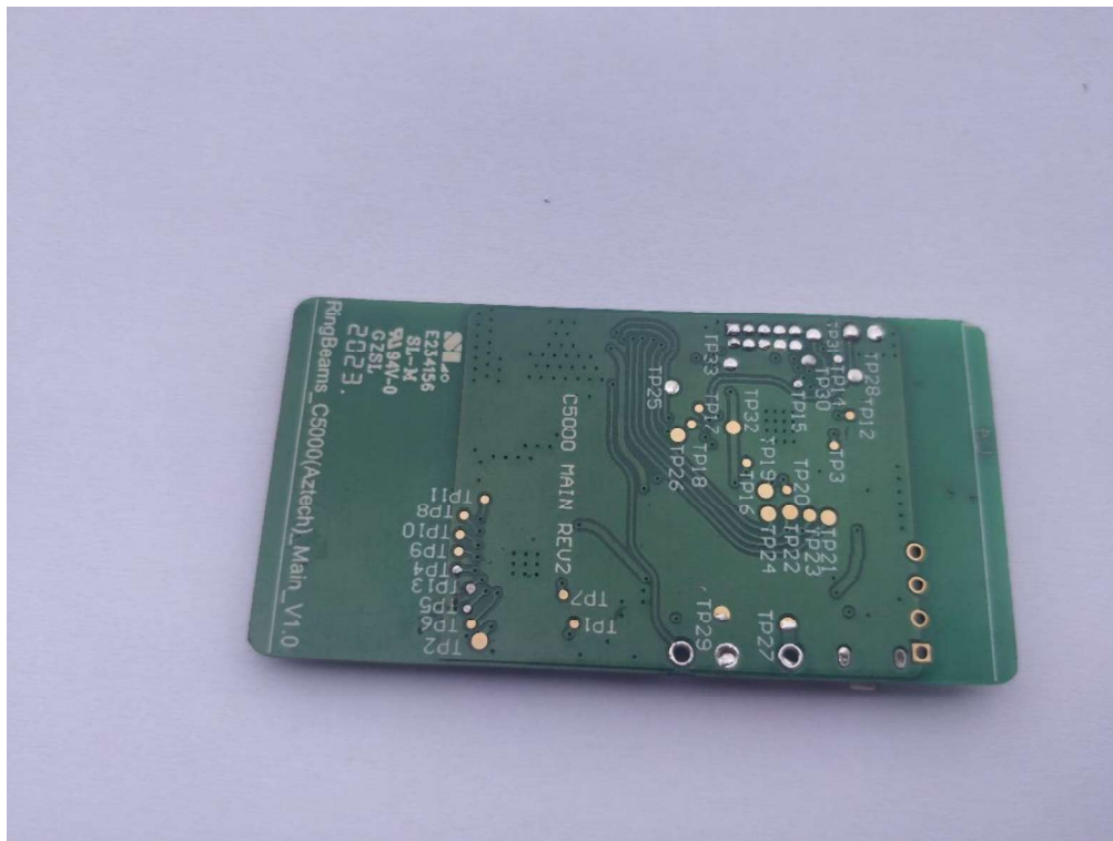
RF PCBA of 5W21S8-A
