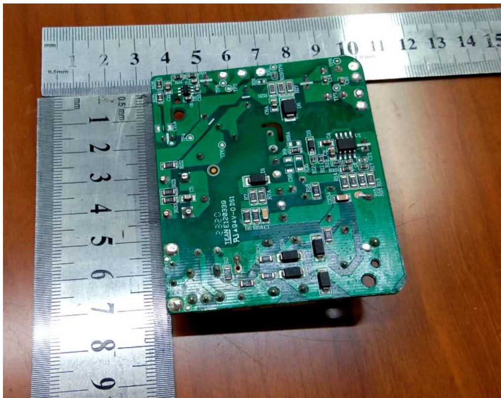
Power PCBA of 5W21S8-A
