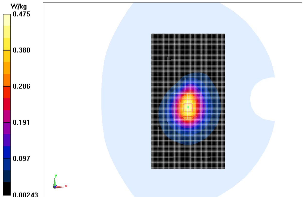
Fig.10 2450 MHz CH11
