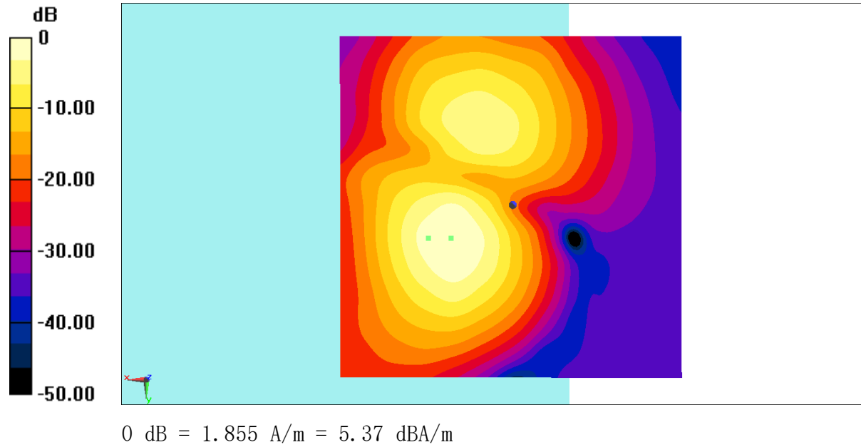
Fig B.12 T-Coil WiFi-5G
