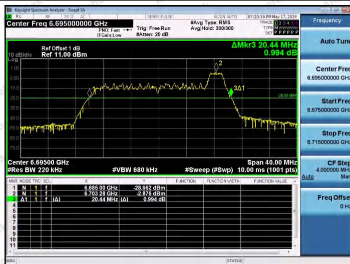
11AX20SISO-Ant1-6695-26Tone-RU8
