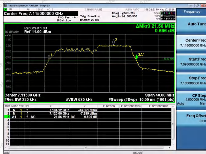
11AX20SISO-Ant1-7115-106Tone-RU54
