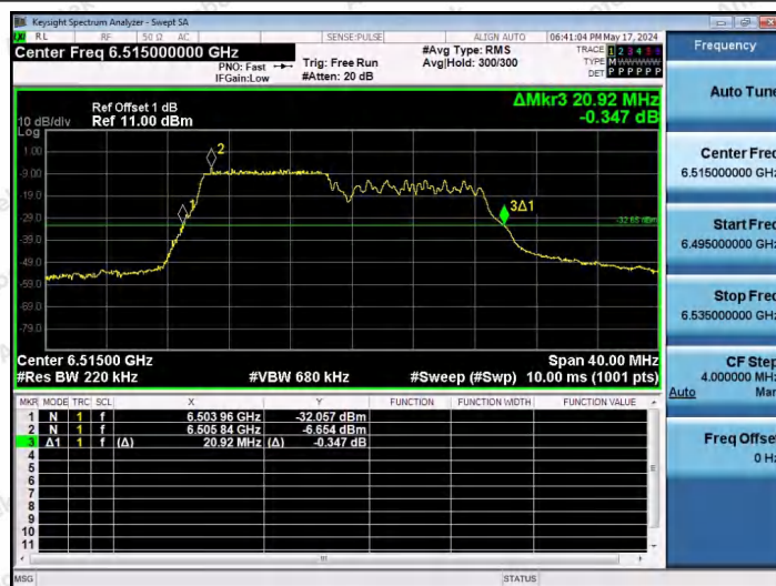
11AX20SISO-Ant1-6515-106Tone-RU53
