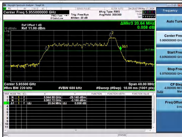
11AX20SISO-Ant1-5955-26Tone-RU8
