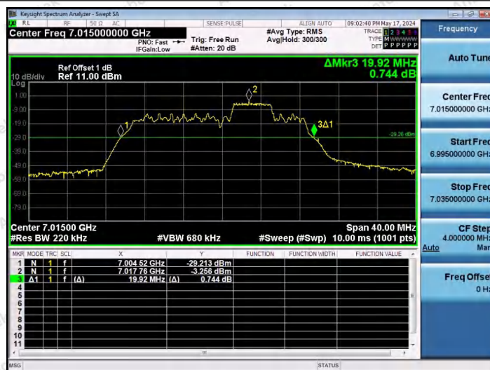
11AX20SISO-Ant1-7015-52Tone-RU39
