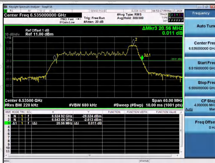
11AX20SISO-Ant1-6535-26Tone-RU8
