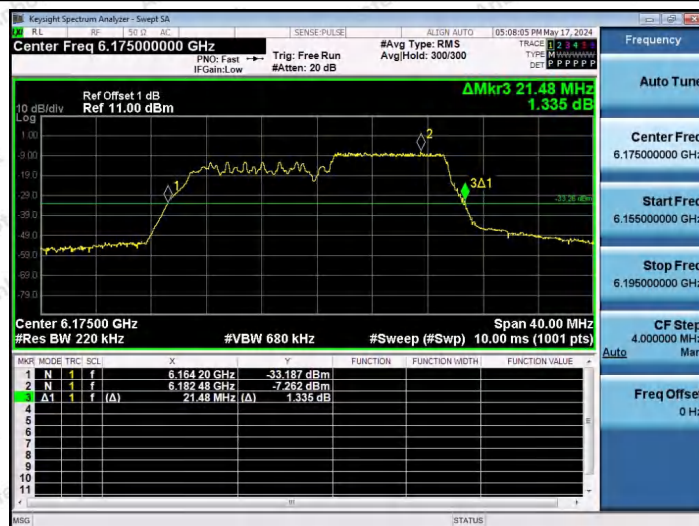
11AX20SISO-Ant1-6175-106Tone-RU54
