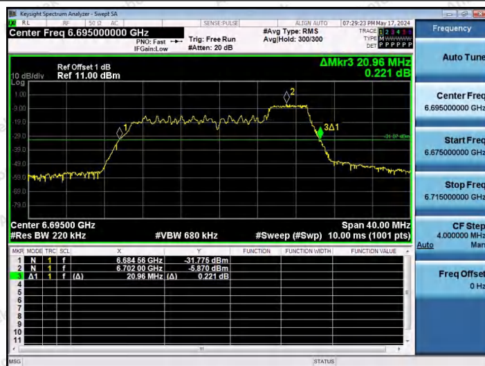
11AX20SISO-Ant1-6695-52Tone-RU40
