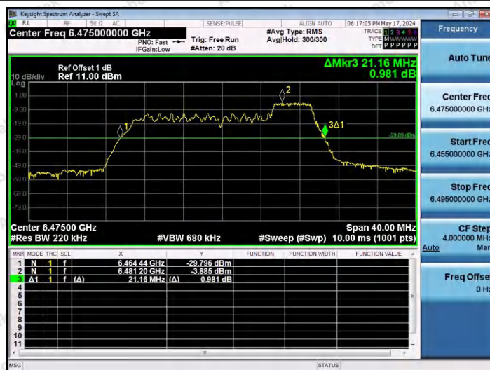
11AX20SISO-Ant1-6475-52Tone-RU40
