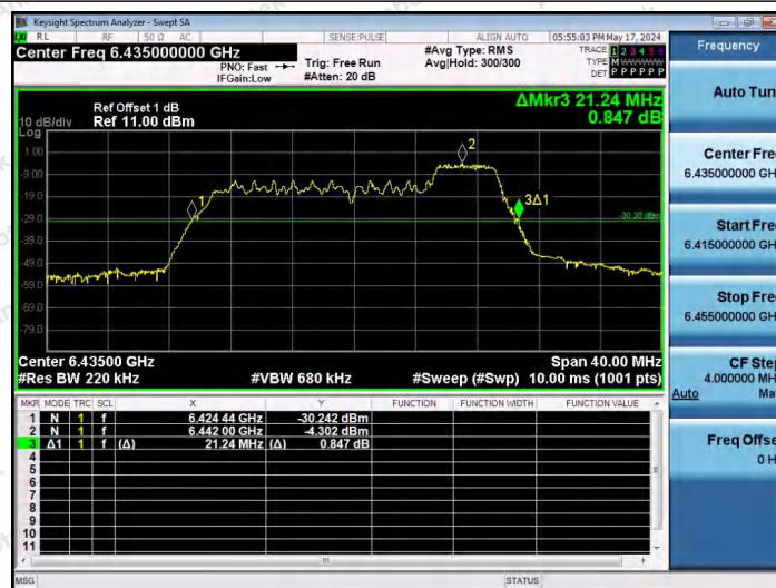
11AX20SISO-Ant1-6435-52Tone-RU40
