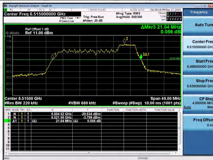
11AX20SISO-Ant1-6515-52Tone-RU40
