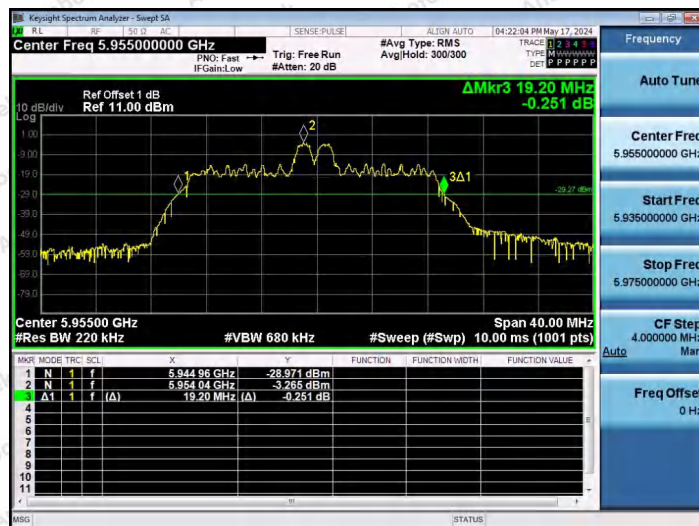
11AX20SISO-Ant1-5955-26Tone-RU4
