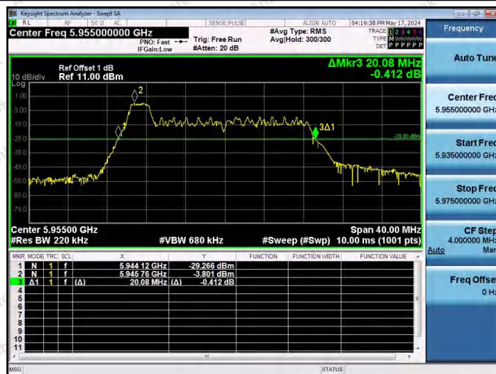
11AX20SISO-Ant1-5955-26Tone-RU0
