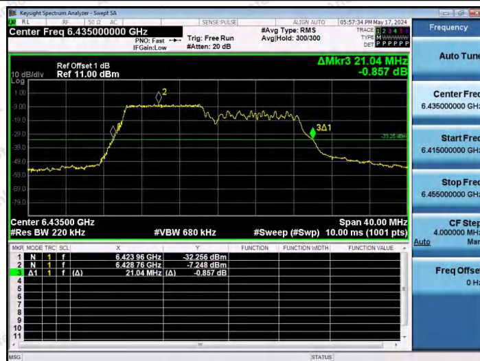
11AX20SISO-Ant1-6435-106Tone-RU53
