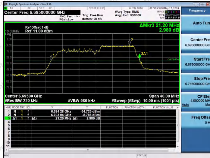
11AX20SISO-Ant1-6695-106Tone-RU54
