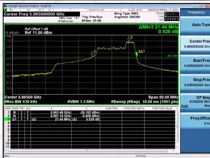
11AX40SISO-Ant1-5965-52Tone-RU44
