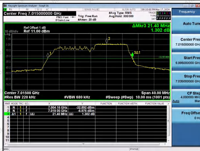
11AX20SISO-Ant1-7015-106Tone-RU54
