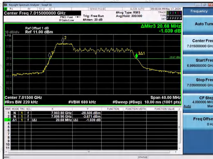
11AX20SISO-Ant1-7015-52Tone-RU37
