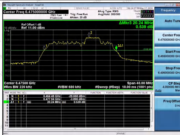
11AX20SISO-Ant1-6475-52Tone-RU39
