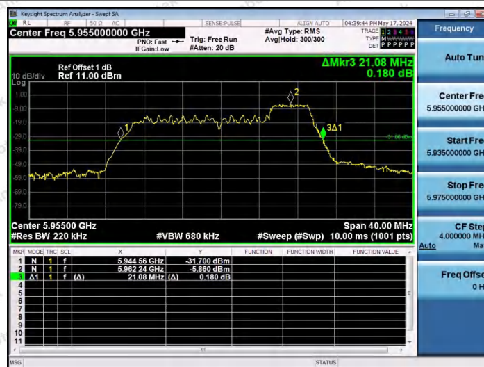
11AX20SISO-Ant1-5955-52Tone-RU40
