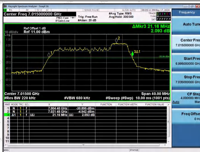
11AX20SISO-Ant1-7015-52Tone-RU40
