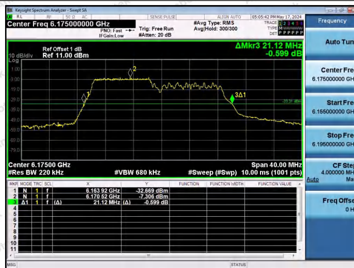
11AX20SISO-Ant1-6175-106Tone-RU53
