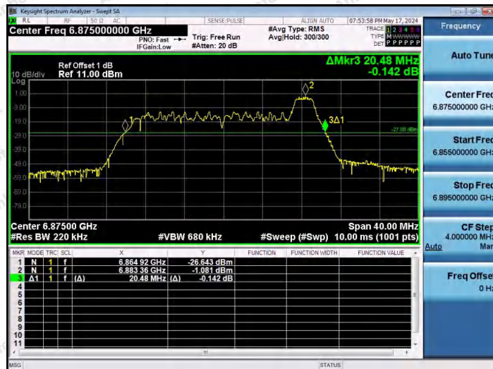
11AX20SISO-Ant1-6875-26Tone-RU8
