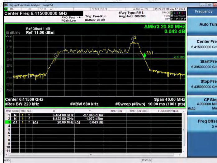
11AX20SISO-Ant1-6415-26Tone-RU8
