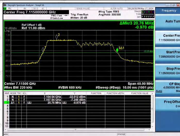
11AX20SISO-Ant1-7115-106Tone-RU53
