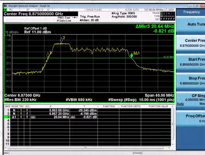
11AX20SISO-Ant1-6875-52Tone-RU37
