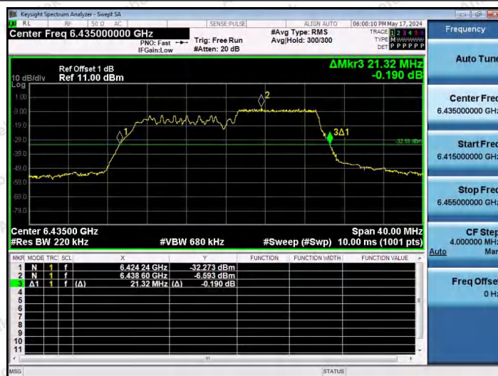
11AX20SISO-Ant1-6435-106Tone-RU54
