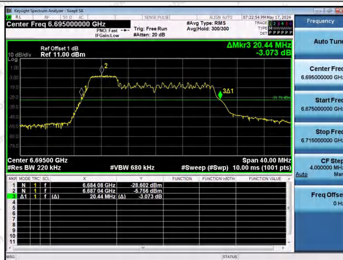
11AX20SISO-Ant1-6695-52Tone-RU37
