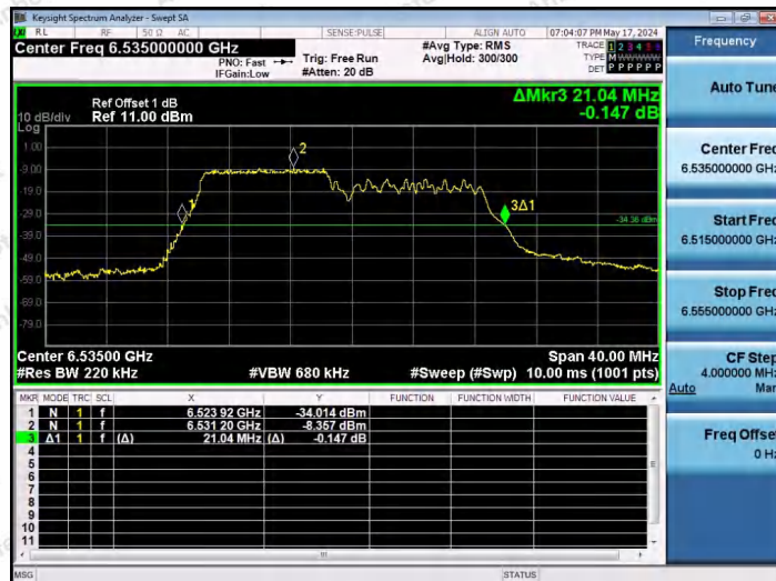
11AX20SISO-Ant1-6535-106Tone-RU53
