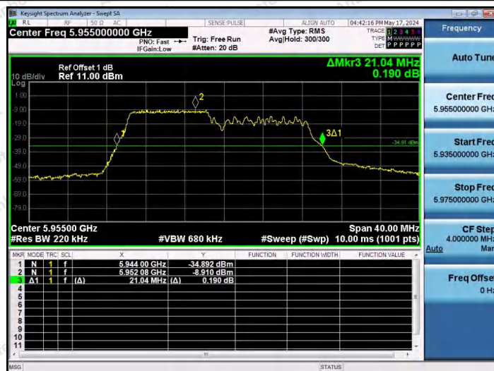
11AX20SISO-Ant1-5955-106Tone-RU53
