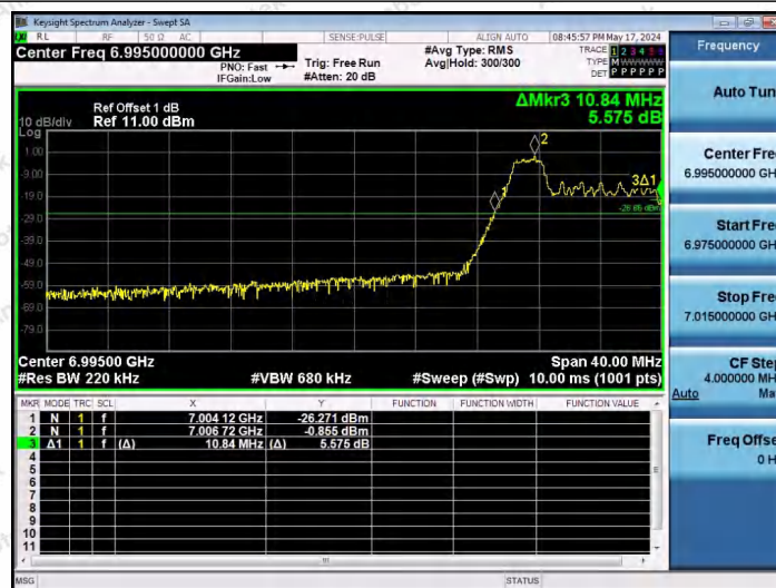
11AX20SISO-Ant1-6995-26Tone-RU0
