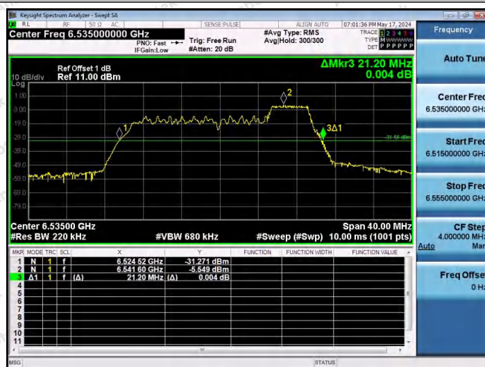
11AX20SISO-Ant1-6535-52Tone-RU40
