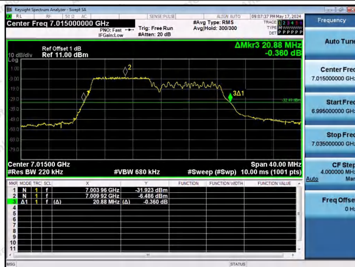
11AX20SISO-Ant1-7015-106Tone-RU53
