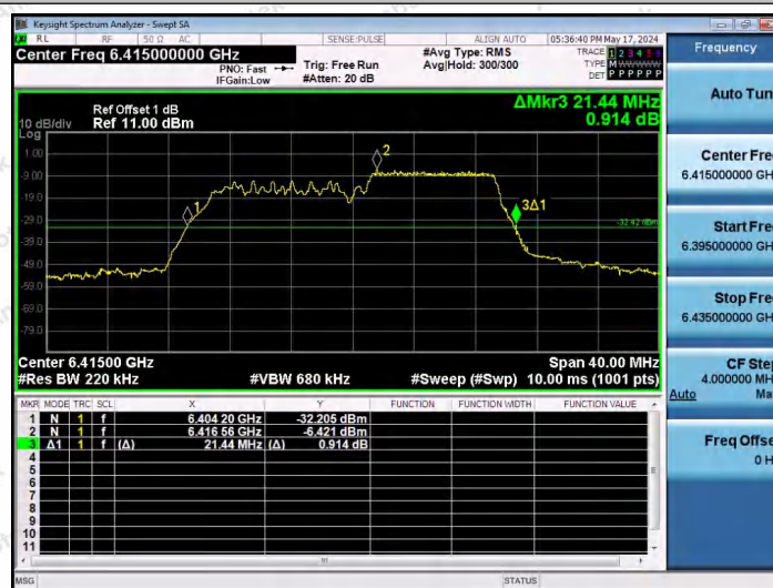
11AX20SISO-Ant1-6415-106Tone-RU54
