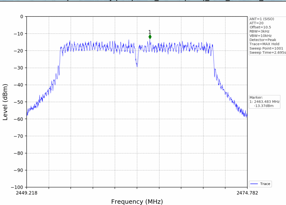
Maximum Power Spectral Density (PSD) NTVN_802.11n(HT20)_SISO_2462MHz_ANT1
