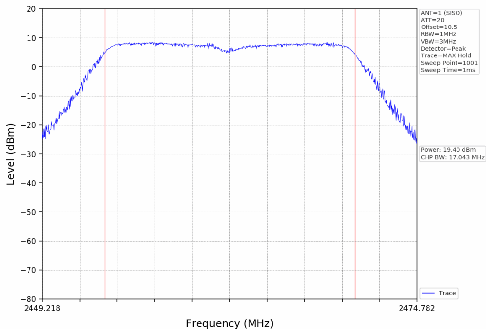
Maximum Conducted Outpower NTN 802.11n(HT20) SISO 2462MHz ANT1
