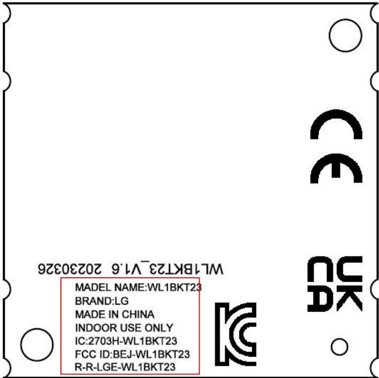
Label Placement Location (EUT Bottom View)
