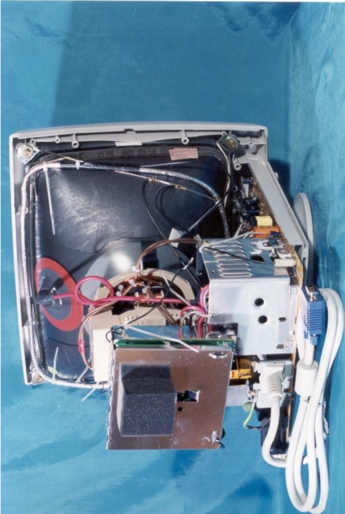
Side View w/o Back Cover
