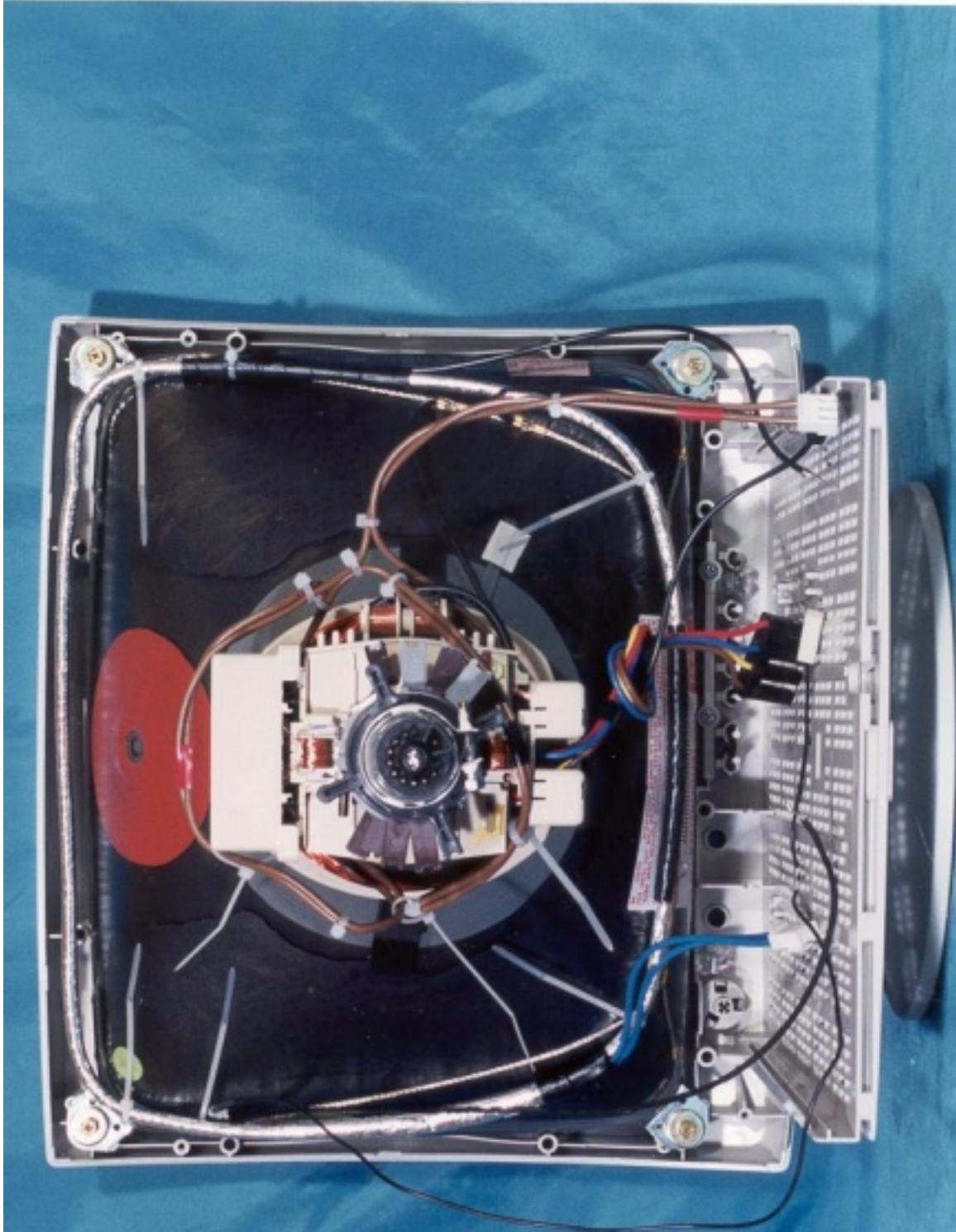
CRT Assembly
