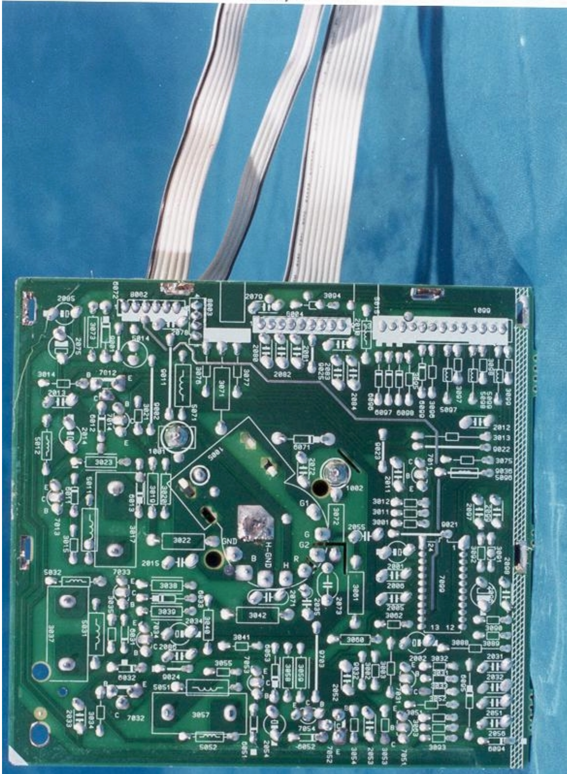
PCB Layout
