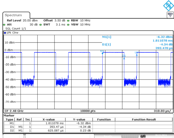
BLE_1M_High_Channel
