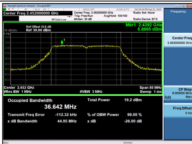
11N40MIMO-Ant2-2452
