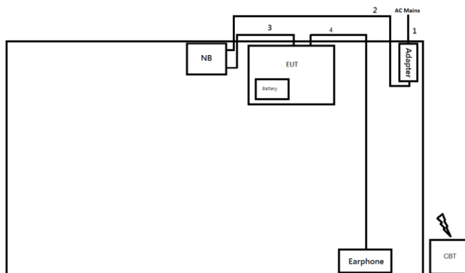
Test Setup Diagram – AC Line Conducted Emission Test - USB Mode
