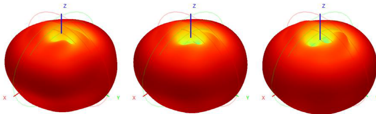
Antenna 3D-2400/2450/2500MHz
