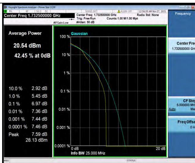
Band4-10MHz-16QAM-20175-27RB#0
