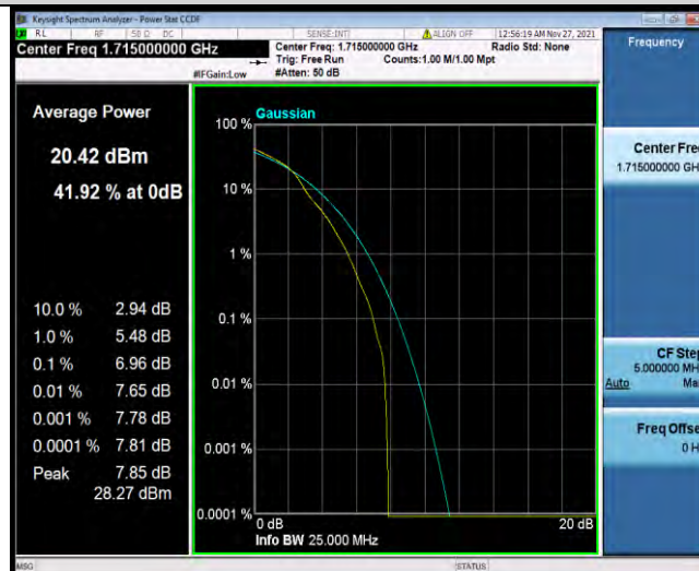
Band4-10MHz-16QAM-20000-27RB#0
