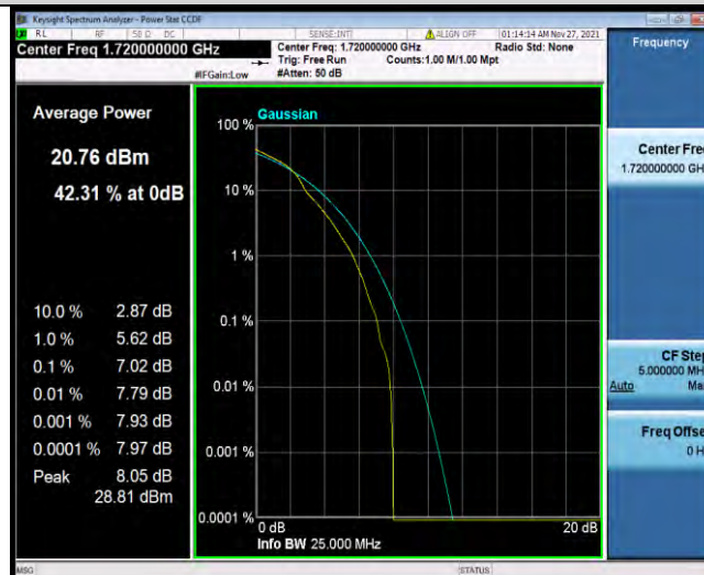
Band4-20MHz-16QAM-20050-27RB#0
