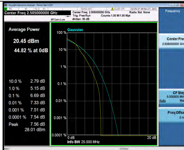
Band7-10MHz-16QAM-20800-27RB#0
