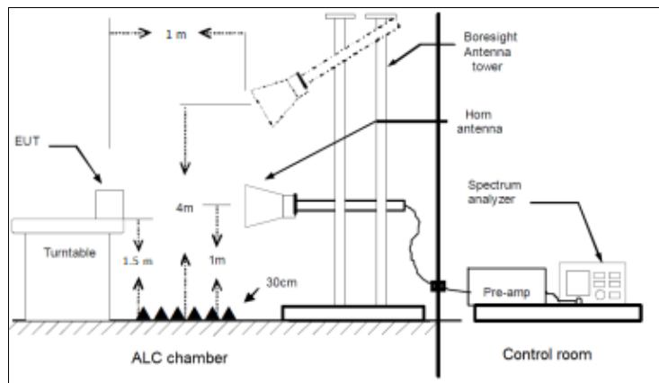
Radiated measurements setup f > 18 \text{ GHz}
