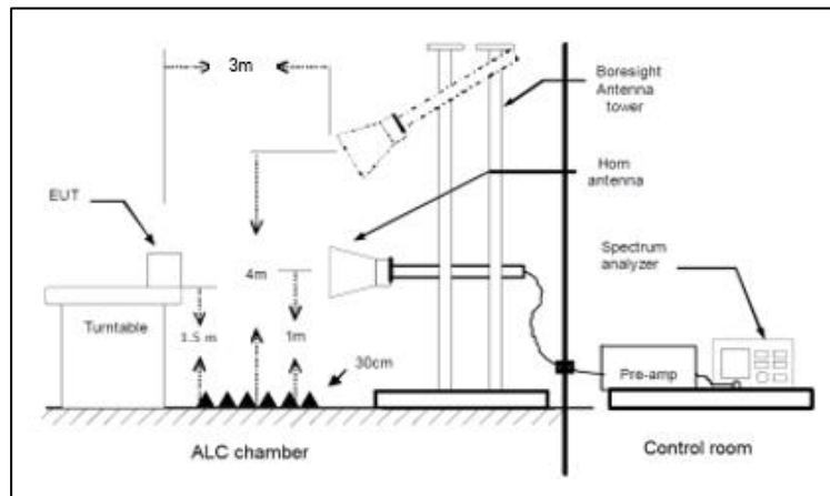
Radiated measurements setup f > 1-18 \text{ GHz}
