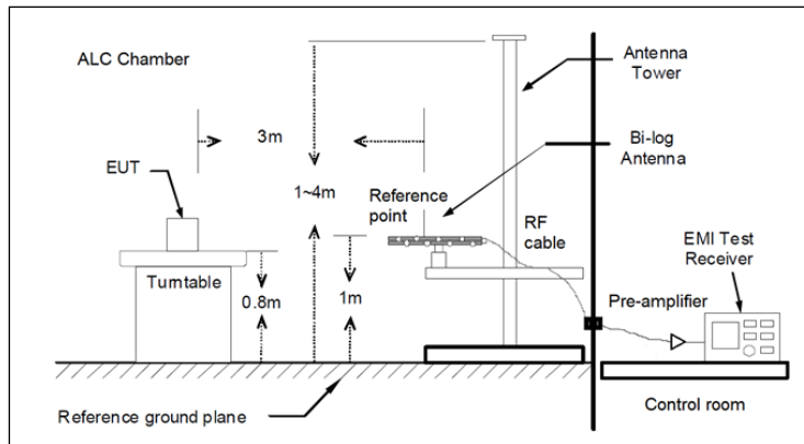
Radiated measurements Setup f < 1 \text{ GHz}
