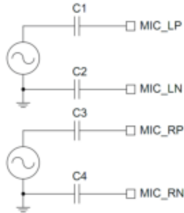
Figure 16: Single-ended Input
