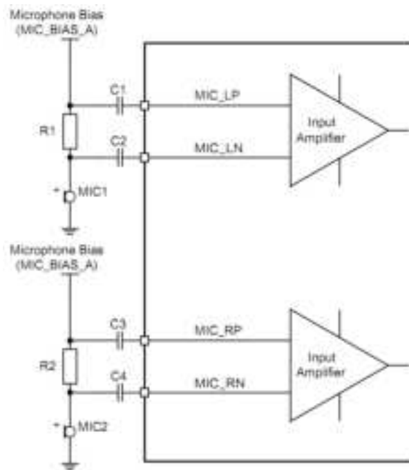
Figure 14: Microphone Biasing
