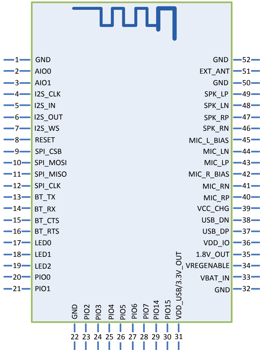
Figure 3: FSC-BT806A PIN Diagram(Top View)
