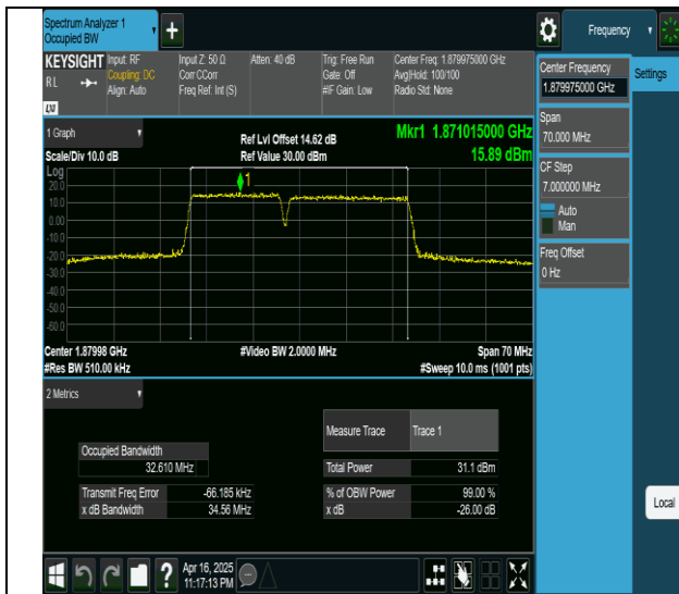
2-2-15MHz-20MHz-QPSK-QPSK-18803-18974-75RB#0- 100RB#0-PASS
