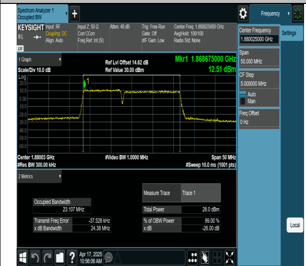
2-2-10MHz-15MHz-256QAM-256QAM-18829-18949-50RB#0- 75RB#0-PASS
