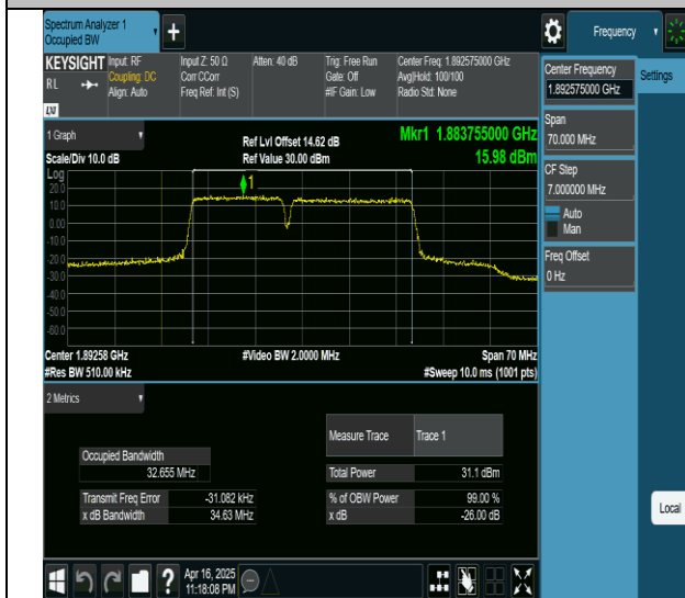
2-2-15MHz-20MHz-QPSK-QPSK-18929-19100-75RB#0- 100RB#0-PASS
