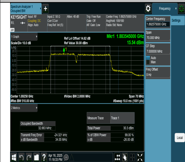
2-2-15MHz-20MHz-16QAM-16QAM-18929-19100-75RB#0- 100RB#0-PASS
