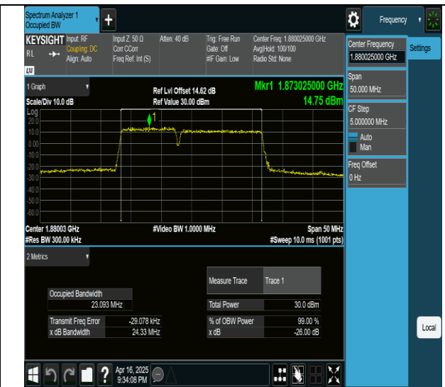
2-2-10MHz-15MHz-16QAM-16QAM-18829-18949-50RB#0- 75RB#0-PASS
