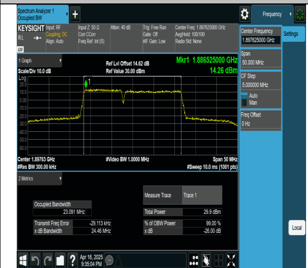
2-2-10MHz-15MHz-16QAM-16QAM-19005-19125-50RB#0- 75RB#0-PASS
