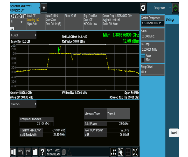
2-2-10MHz-15MHz-256QAM-256QAM-19005-19125-50RB#0-75RB#0-PASS
