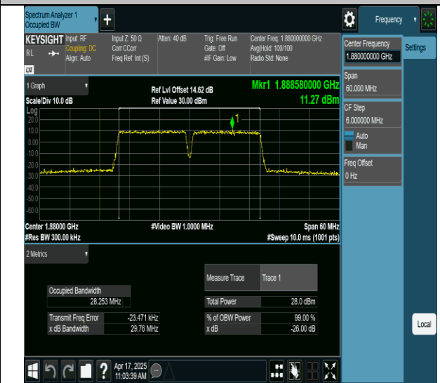
2-2-15MHz-15MHz-256QAM-256QAM-18825-18975-75RB#0- 75RB#0-PASS
