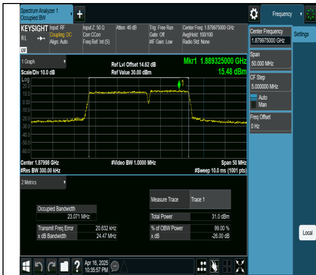
2-2-15MHz-10MHz-QPSK-QPSK-18851-18971-75RB#0-50RB#0-PASS
