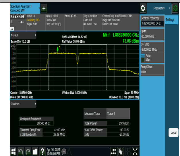
2-2-15MHz-15MHz-16QAM-16QAM-18975-19125-75RB#0- 75RB#0-PASS
