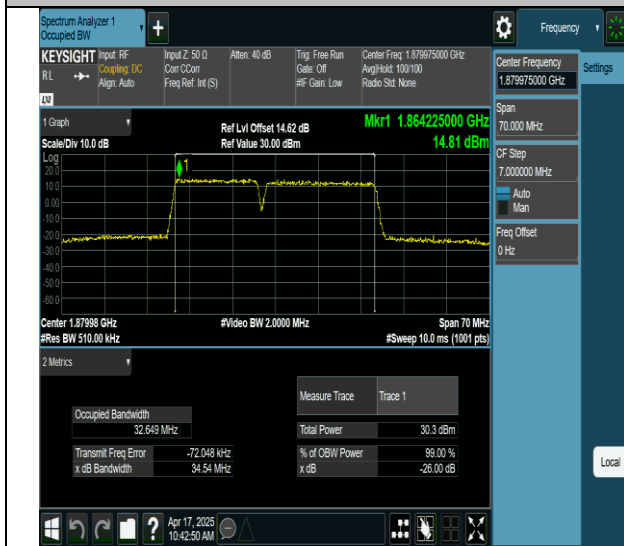
2-2-15MHz-20MHz-64QAM-64QAM-18803-18974-75RB#0- 100RB#0-PASS
