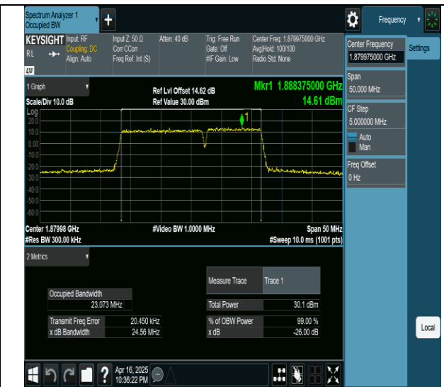
2-2-15MHz-10MHz-16QAM-16QAM-18851-18971-75RB#0-50RB#0-PASS
