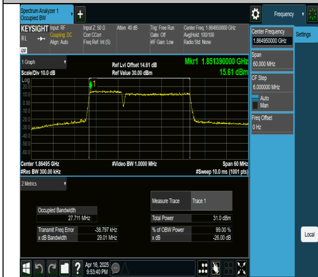
2-2-10MHz-20MHz-QPSK-QPSK-18655-18799-50RB#0-100RB#0-PASS
