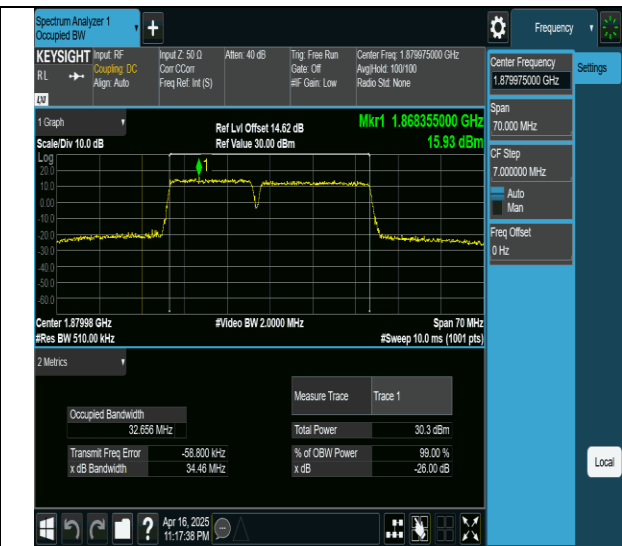
2-2-15MHz-20MHz-16QAM-16QAM-18803-18974-75RB#0- 100RB#0-PASS
