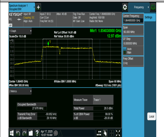
2-2-10MHz-20MHz-256QAM-256QAM-18655-18799-50RB#0-100RB#0-PASS
