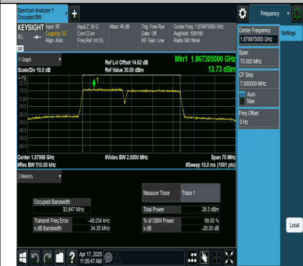
2-2-15MHz-20MHz-256QAM-256QAM-18803-18974-75RB#0- 100RB#0-PASS
