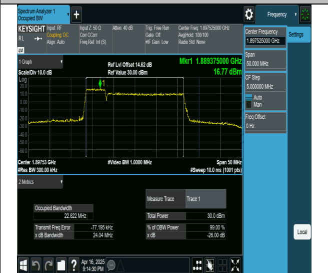
2-2-5MHz-20MHz-16QAM-16QAM-18983-19100-25RB#0- 100RB#0-PASS
