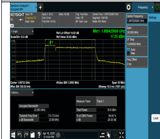
2-2-5MHz-20MHz-QPSK-QPSK-18983-19100-25RB#0-100RB#0- PASS
