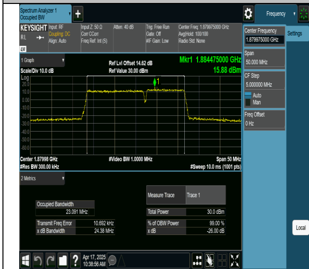
2-2-15MHz-10MHz-64QAM-64QAM-18851-18971-75RB#0-50RB#0-PASS
