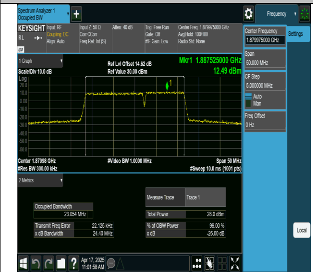
2-2-15MHz-10MHz-256QAM-256QAM-18851-18971-75RB#0-50RB#0-PASS
