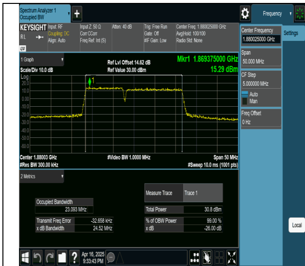
2-2-10MHz-15MHz-QPSK-QPSK-18829-18949-50RB#0-75RB#0- PASS
