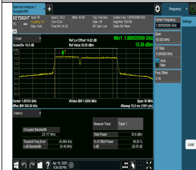
2-2-10MHz-15MHz-QPSK-QPSK-19005-19125-50RB#0-75RB#0- PASS
