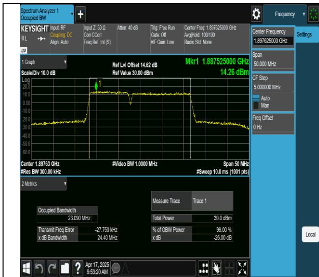
2-2-10MHz-15MHz-64QAM-64QAM-19005-19125-50RB#0-75RB#0-PASS
