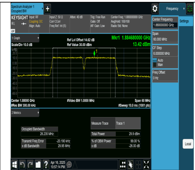
2-2-15MHz-15MHz-16QAM-16QAM-18825-18975-75RB#0- 75RB#0-PASS
