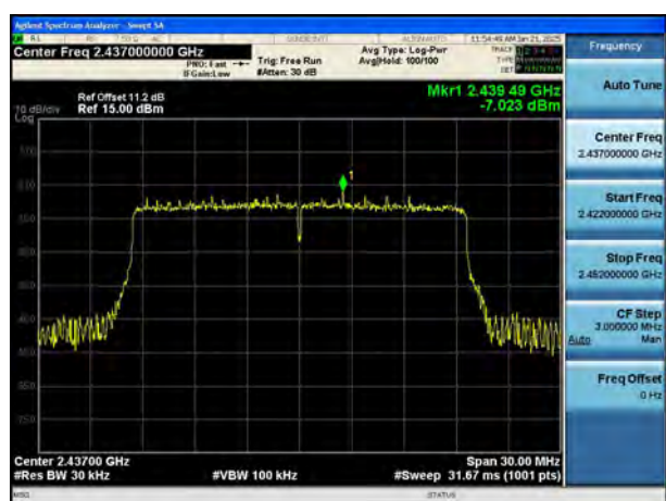
Mode:802.11ax HE20 Tone:242T Frequency:2437MHz Ant:Chain0
