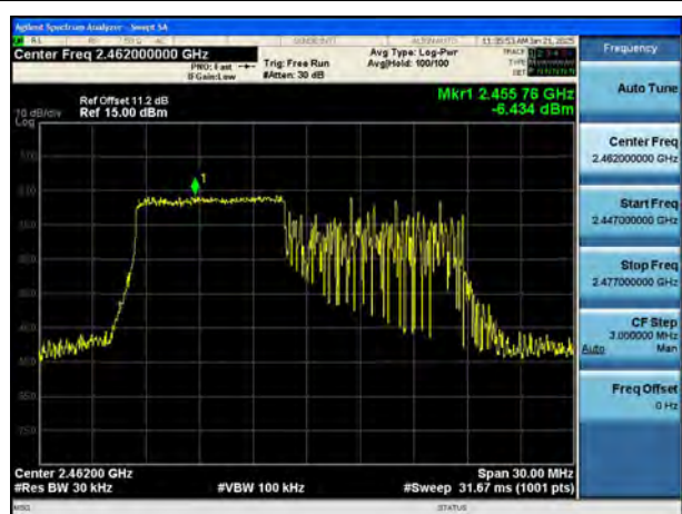
Mode:802.11ax HE20 Tone:106T Frequency:2462MHz Ant:Chain0
