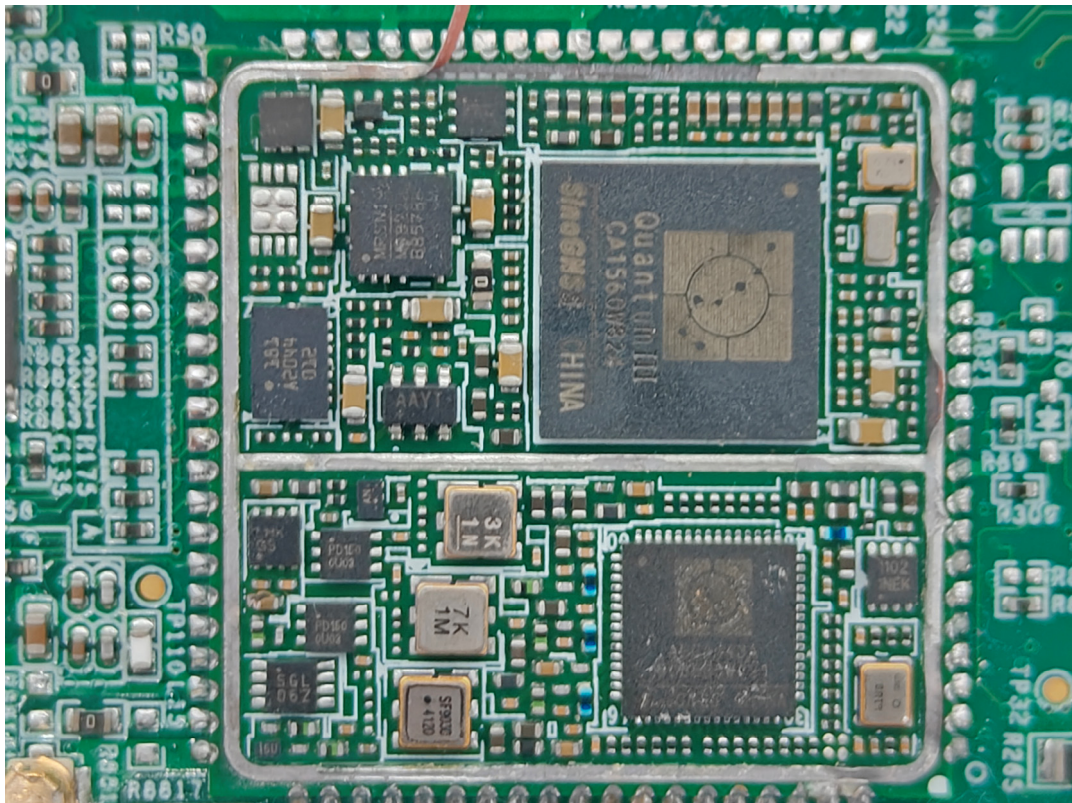
GNSS Module unshielded
