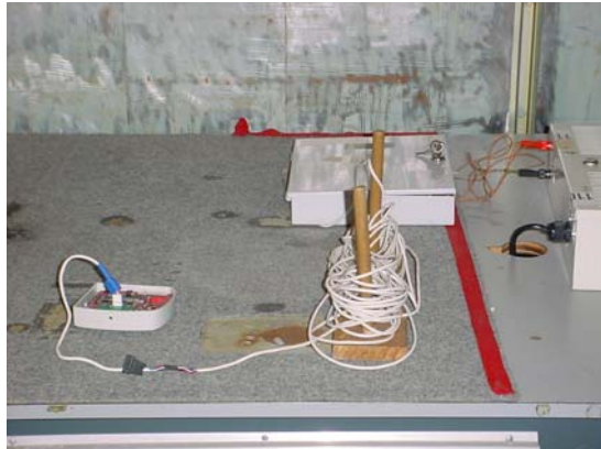
Conducted emissions test set up
