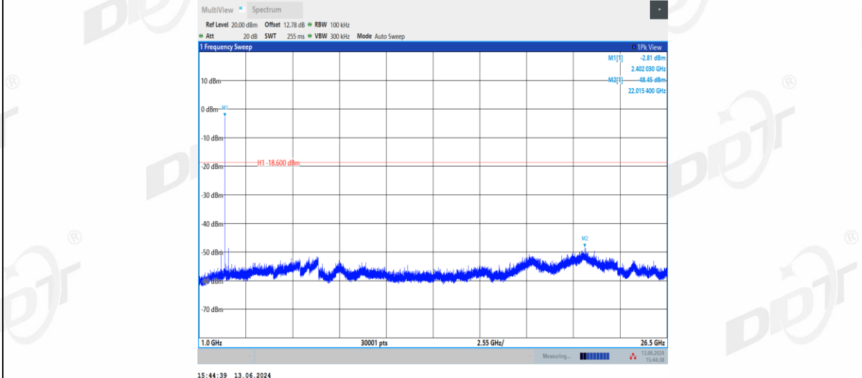
3DH5_Right side_2402_0~Reference
