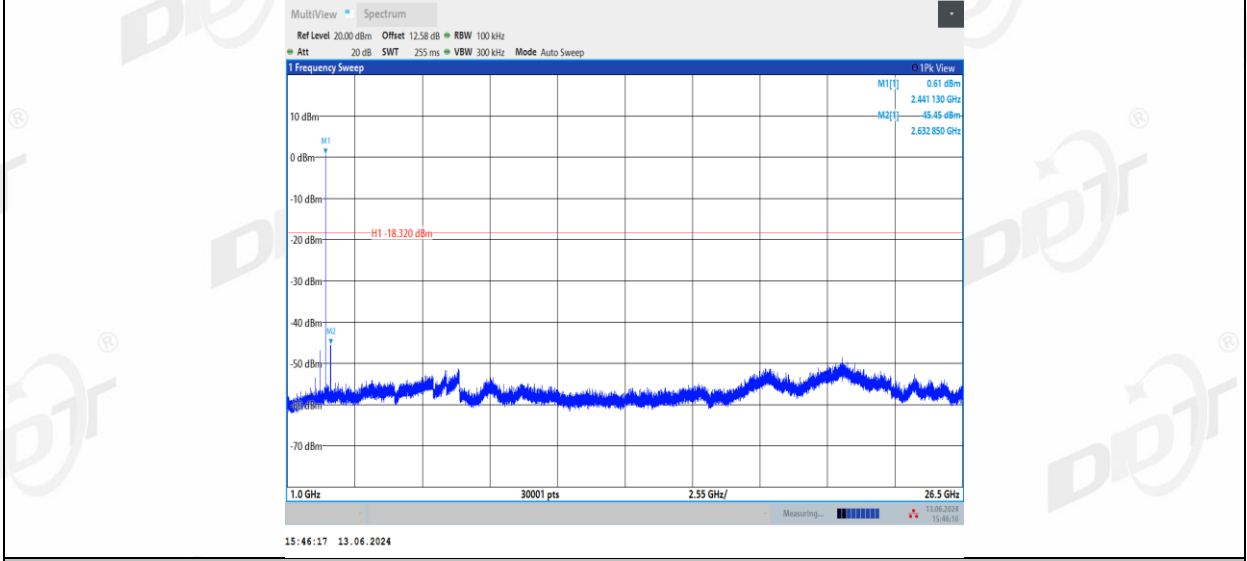
3DH5_Right side_2441_0~Reference
