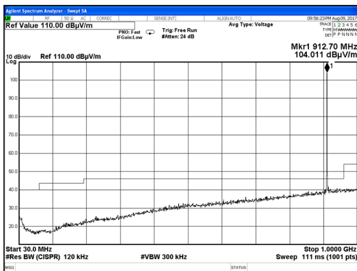
Plot 7.6.10 Radiated emission measurements from 30 to 1000 MHz at the mid carrier frequency
