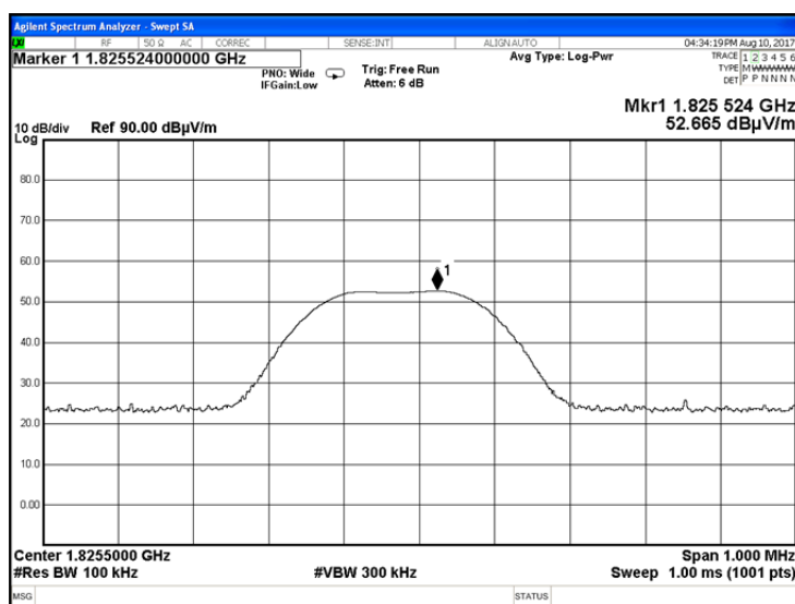
Plot 7.6.16 Radiated emission measurements at the second harmonic of low carrier frequency
