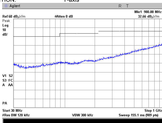
Plot 8.1.4 Radiated emission measurements in 30 - 1000 MHz range, horizontal antenna polarization
