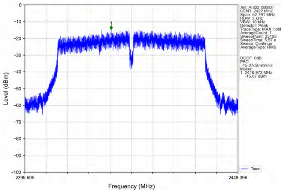
802.11ac(VHT40)_LCH_2422MHz_Ant22 (SISO)_NTNV
