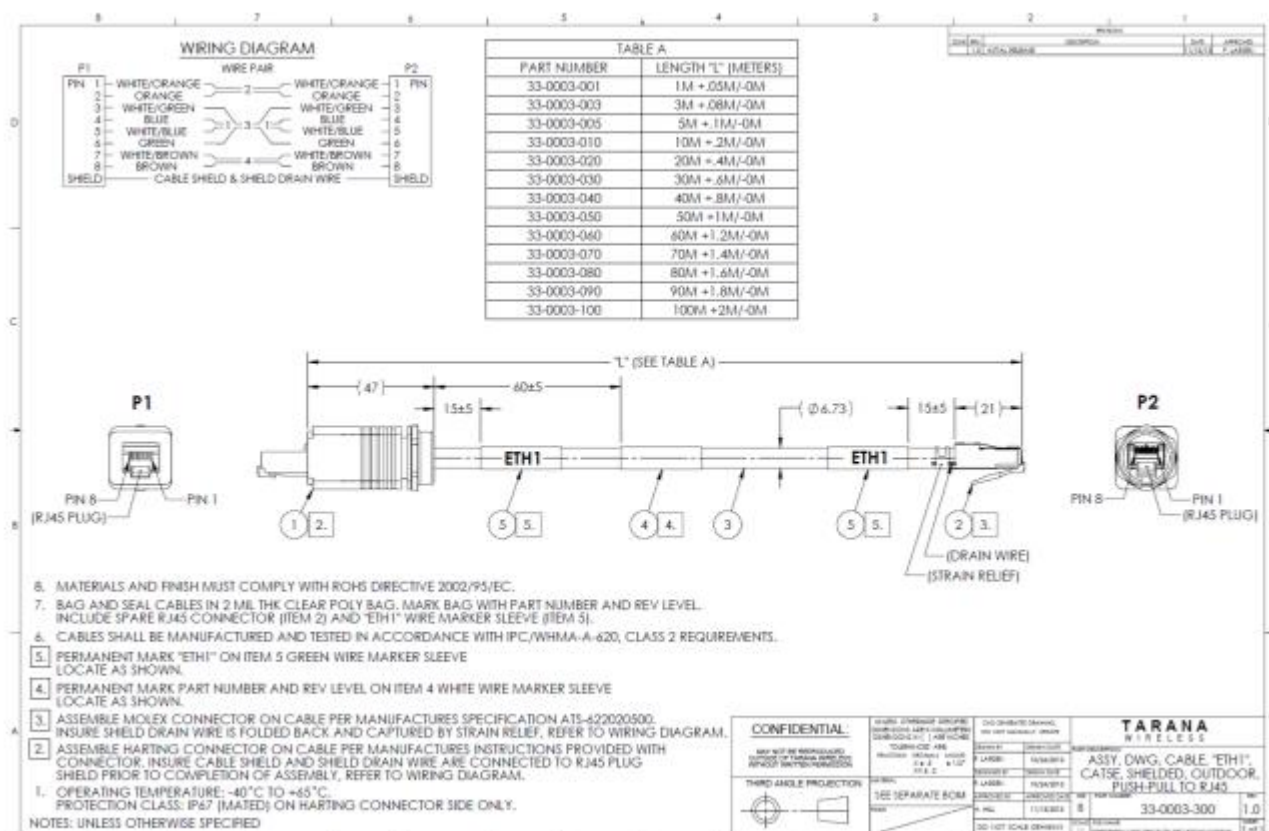
Figure 9: and Gen 2 EN_M, EN_S, and CN Lite RJ-45 "ETH1" Cable Drawing
