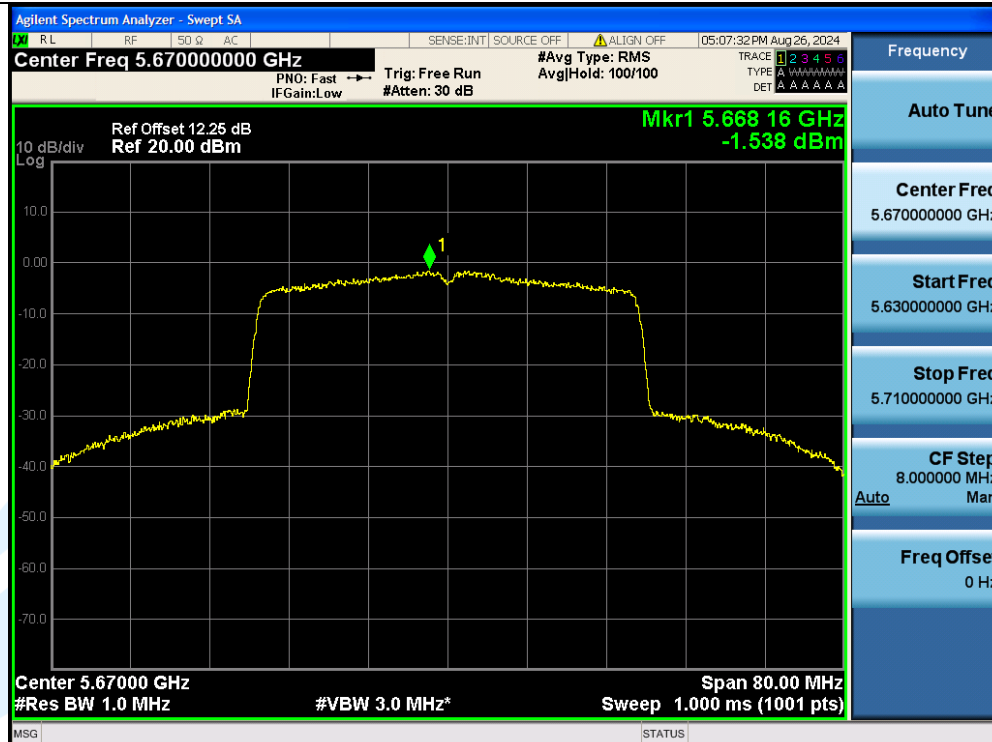
11AX40MIMO-Ant3-5670-PASS
