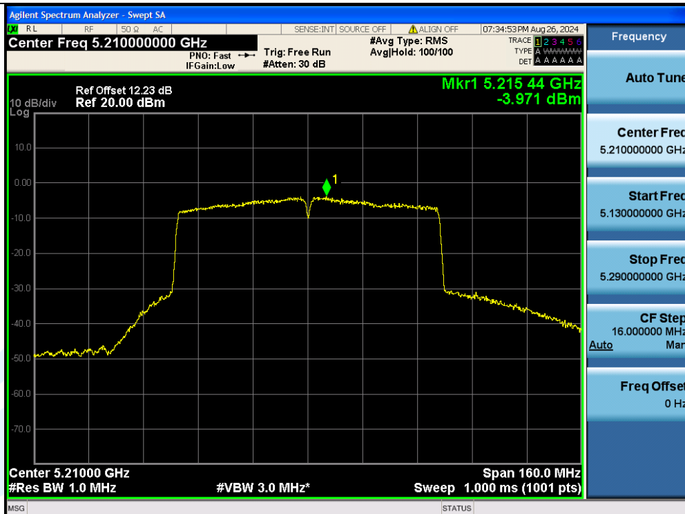
11AC80MIMO-Ant2-5210-PASS
