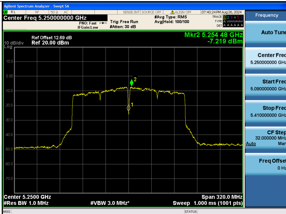
11AC160MIMO-Ant2-5250 UNII-2A-PASS
