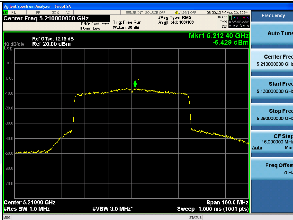
11AX80MIMO-Ant2-5210-PASS
