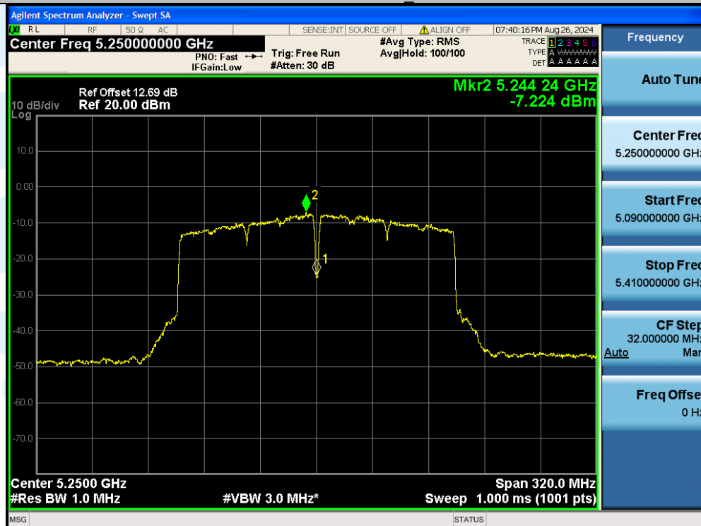
11AC160MIMO-Ant3-5250_UNII-2A-PASS
