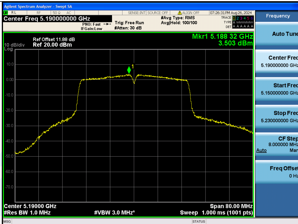
11AC40MIMO-Ant2-5190-PASS
