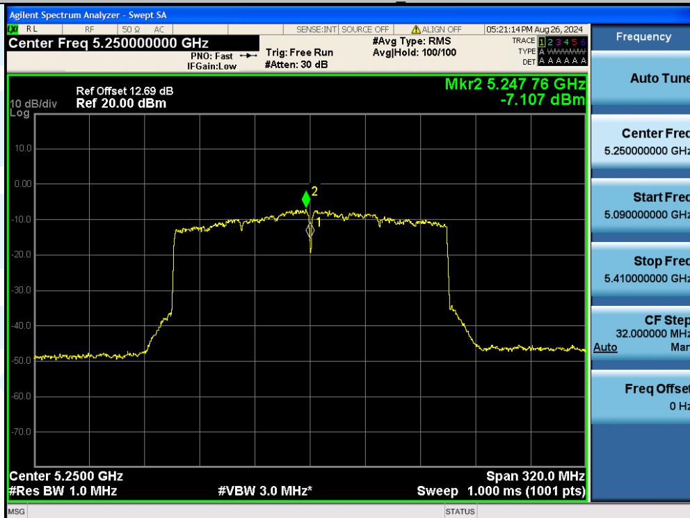
11AX160MIMO-Ant3-5250_UNII-2A-PASS
