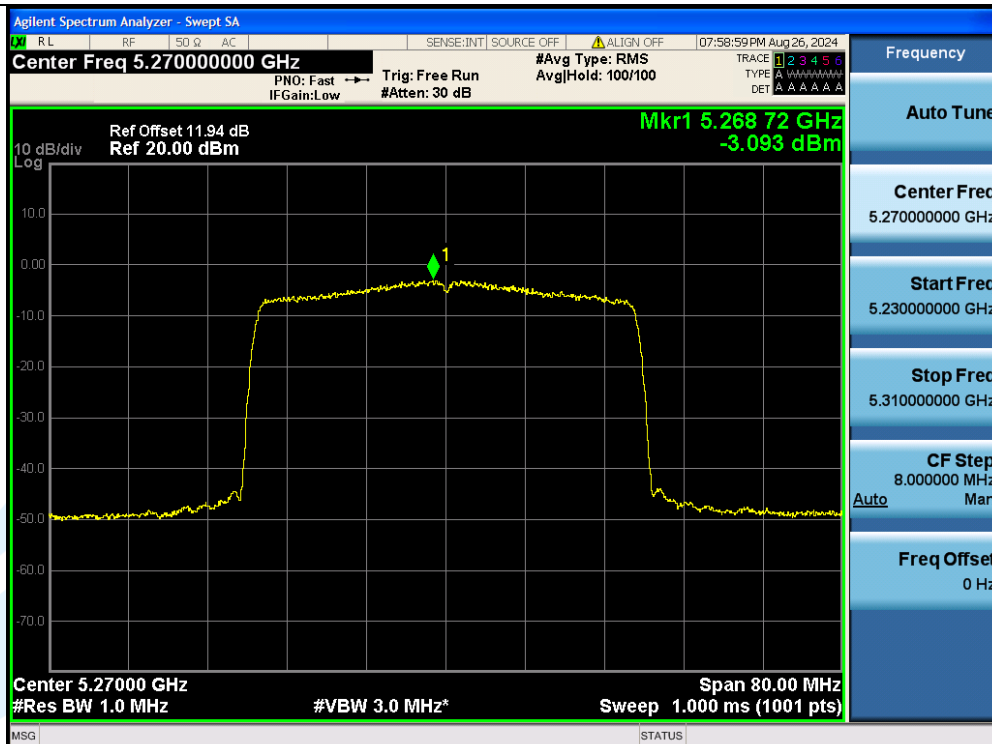
11AX40MIMO-Ant2-5270-PASS
