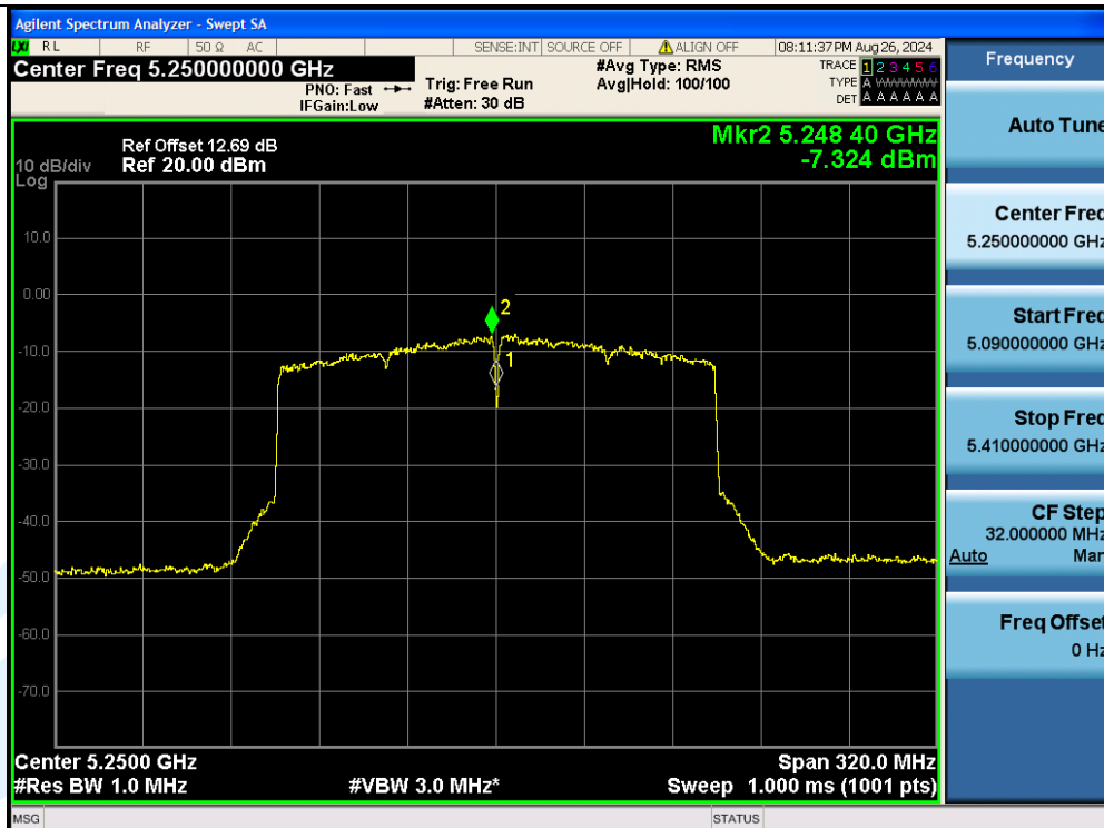
11AX160MIMO-Ant2-5250_UNII-1-PASS
