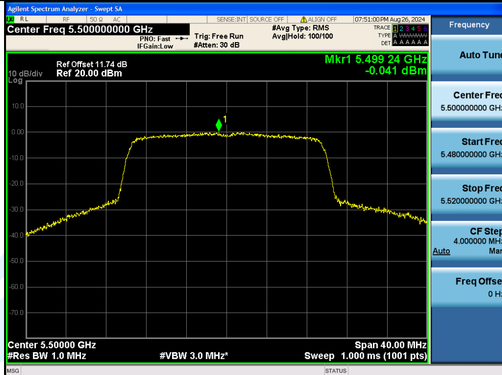
11AX20MIMO-Ant2-5500-PASS
