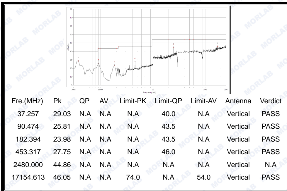
(30MHz to 25GHz, Antenna Vertical @ \pi/4 -DQPSK, channel 78)
