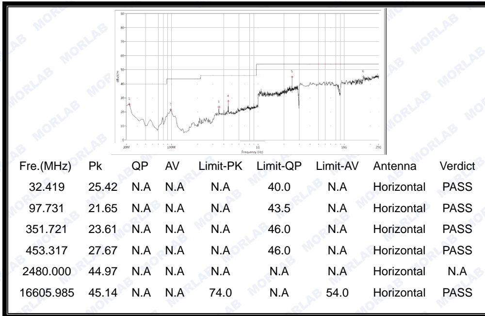
(30MHz to 25GHz, Antenna Horizontal @ GFSK, channel 78)
