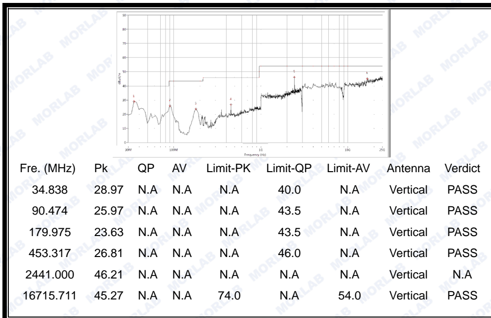
(30MHz to 25GHz, Antenna Vertical @ GFSK, channel 39)
