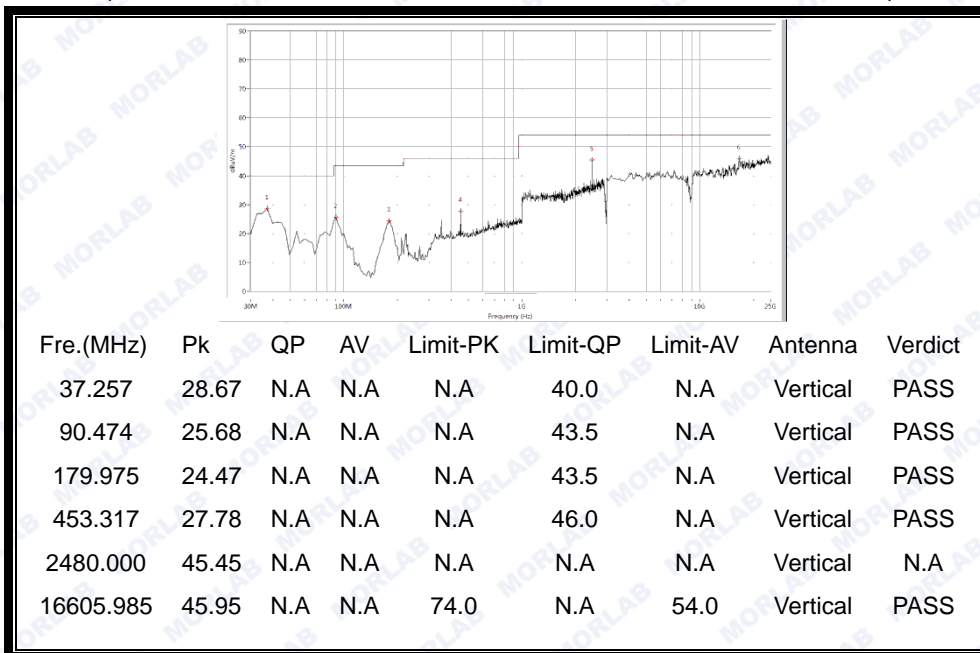
(30MHz to 25GHz, Antenna Vertical @ GFSK, channel 78)
