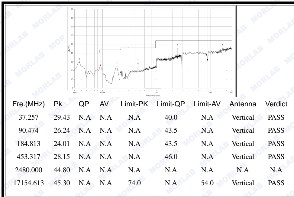
(30MHz to 25GHz, Antenna Vertical @8-DPSK, channel 78)
