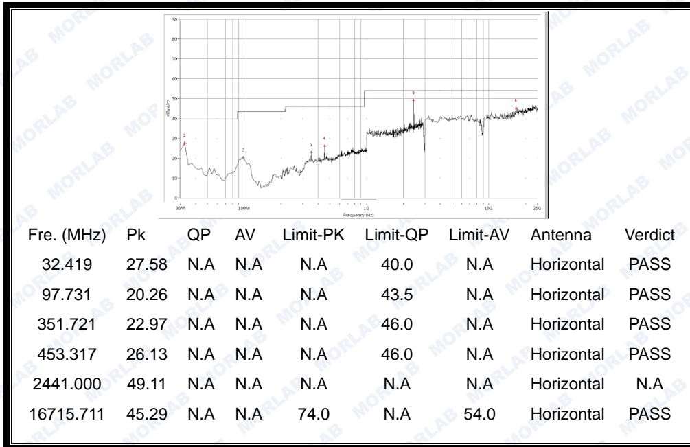
(30MHz to 25GHz, Antenna Horizontal @ GFSK, channel 39)
