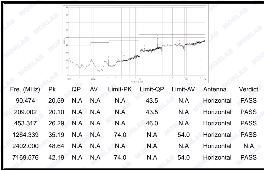
(30MHz to 25GHz, Antenna Horizontal @ \pi/4 -DQPSK, channel 0)
