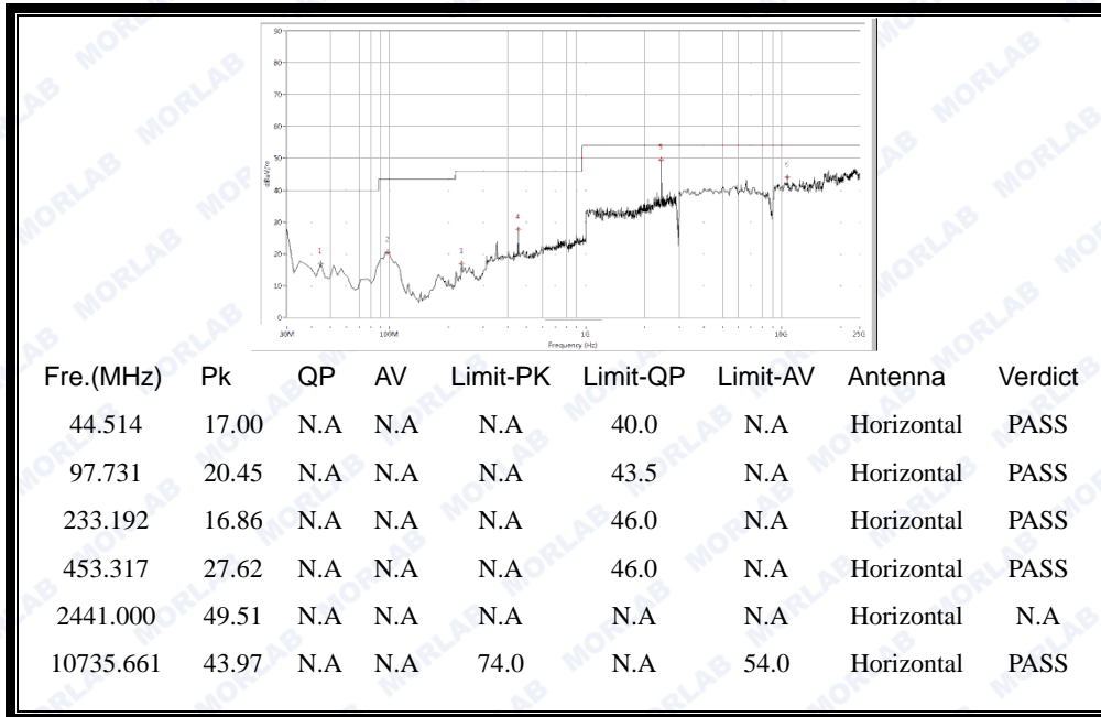
(30MHz to 25GHz, Antenna Horizontal @8-DPSK, channel 39)
