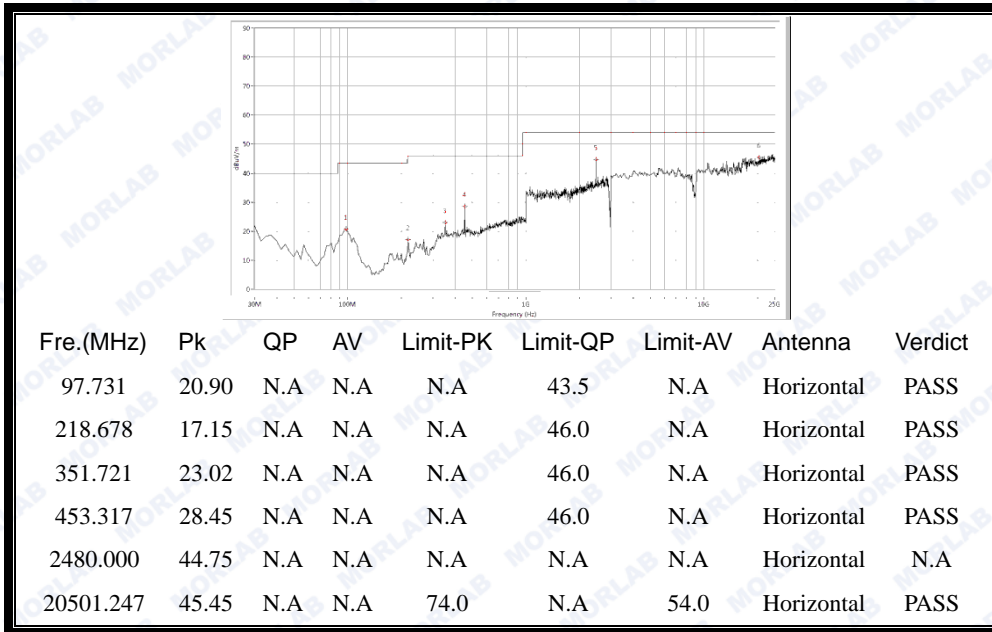
(30MHz to 25GHz, Antenna Horizontal @8-DPSK, channel 78)
