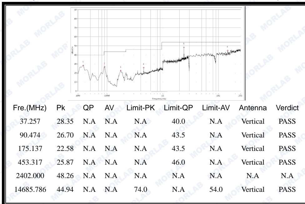
(30MHz to 25GHz, Antenna Vertical @8-DPSK, channel 0)
