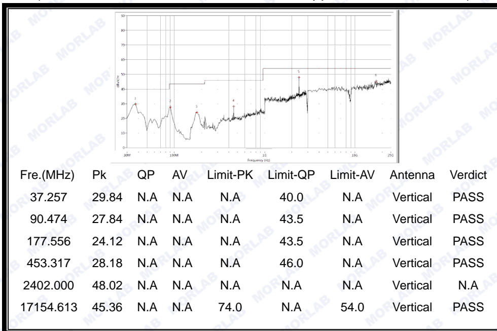
(30MHz to 25GHz, Antenna Vertical @ \pi/4 -DQPSK, channel 0)
