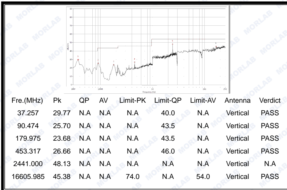
(30MHz to 25GHz, Antenna Vertical @ \pi/4 -DQPSK, channel 39)
