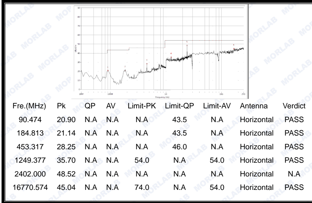
(30MHz to 25GHz, Antenna Horizontal @ GFSK, channel 0)
