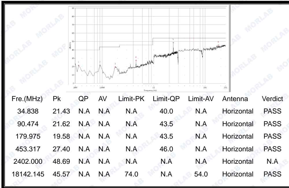
(30MHz to 25GHz, Antenna Horizontal @8-DPSK, channel 0)
