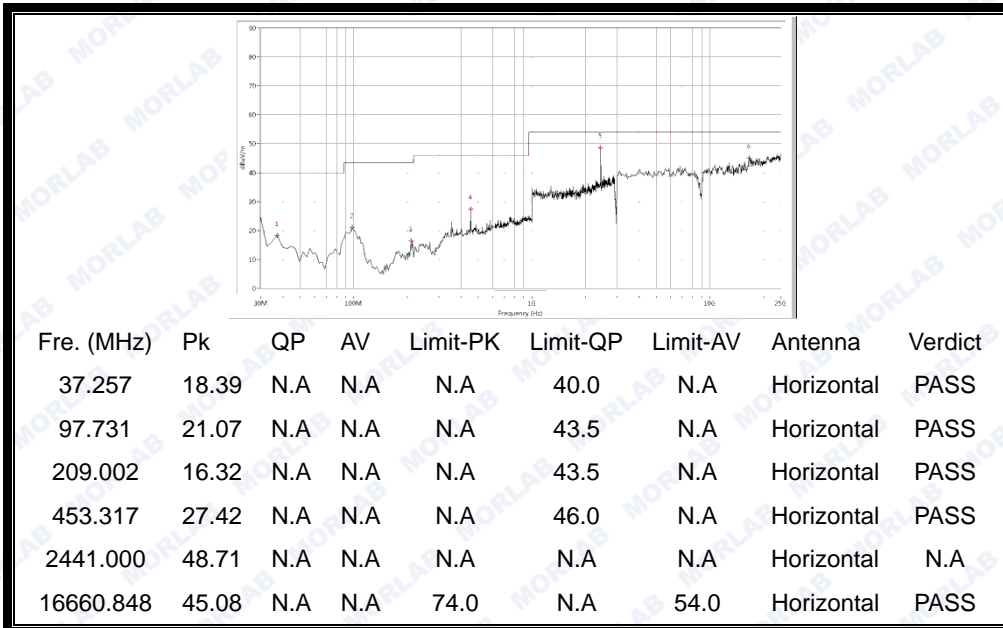
(30MHz to 25GHz, Antenna Horizontal @ \pi/4 -DQPSK, channel 39)
