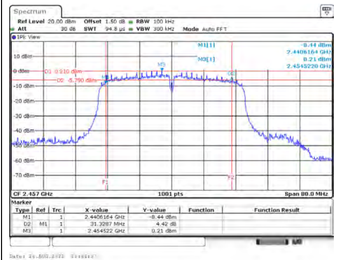
802.11n (40 MHz) / 2457 MHz
