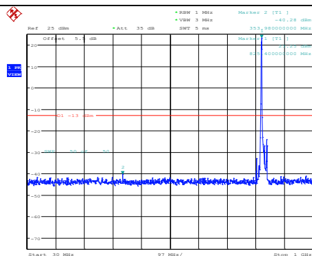
Band5-10MHz-16QAM-20450-1RB#0- Range1:30~1000MHz
