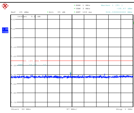
Band7-20MHz-16QAM-20850-1RB#0-Range1:30~1000MHz
