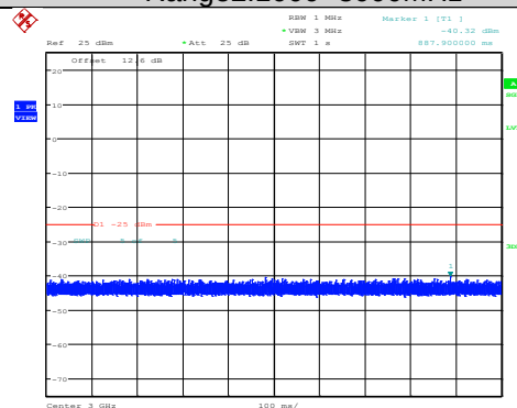
Band7-5MHz-16QAM-21425-1RB#0- Range2:1000~3000MHz
