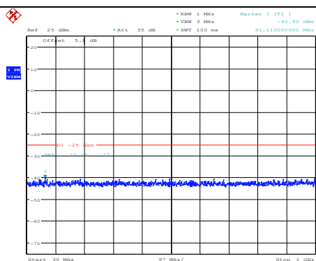
Band7-10MHz-16QAM-20800-1RB#0- Range1:30~1000MHz
