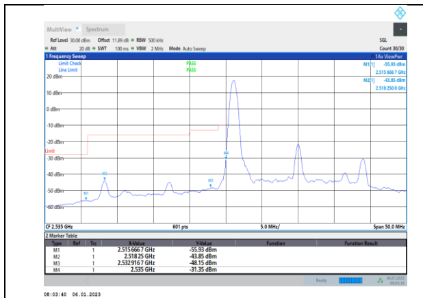
Band41-20MHz-64QAM-40140-100RB#0
