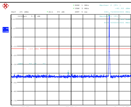
Band5-3MHz-64QAM-20415-1RB#0- Range1:30~1000MHz
