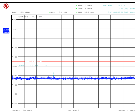
Band7-5MHz-64QAM-21425-1RB#0- Range1:30~1000MHz
