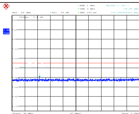
Band7-5MHz-16QAM-21100-1RB#0- Range1:30~1000MHz
