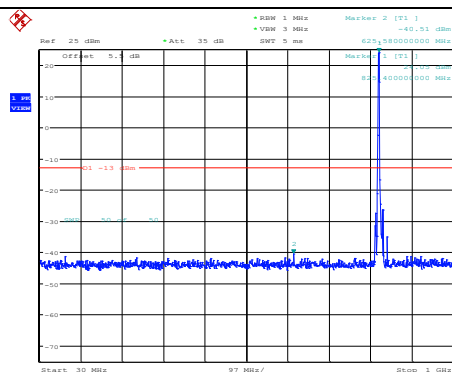
Band5-5MHz-QPSK-20425-1RB#0- Range1:30~1000MHz
