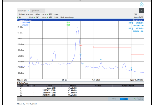
Band41-20MHz-64QAM-41140-100RB#0
