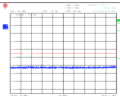
Band7-10MHz-16QAM-21100-1RB#0- Range1:30~1000MHz
