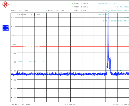
Band5-10MHz-QPSK-20450-1RB#0- Range1:30~1000MHz
