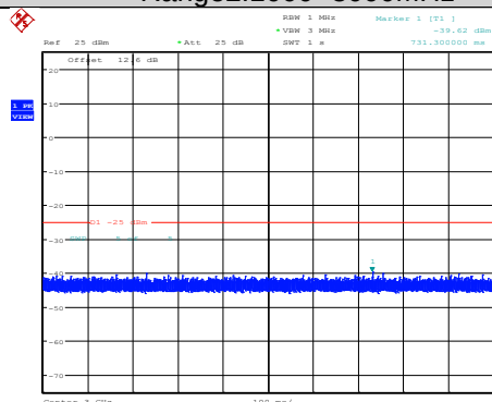
Band7-20MHz-16QAM-21350-1RB#0-Range2:1000~3000MHz
