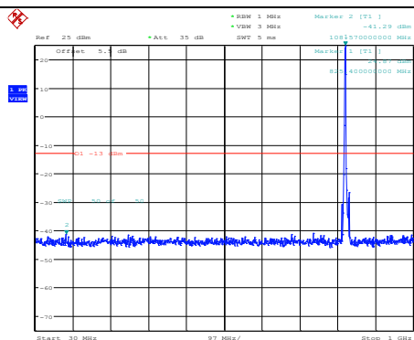
Band5-5MHz-16QAM-20425-1RB#0- Range1:30~1000MHz
