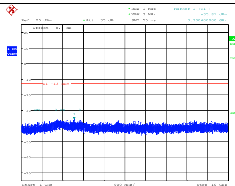
Band5-5MHz-64QAM-20525-1RB#0- Range2:1000~10000MHz
