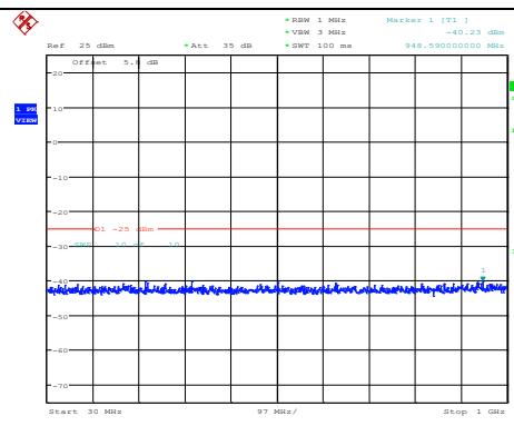
Band7-20MHz-16QAM-21100-1RB#0-Range1:30~1000MHz
