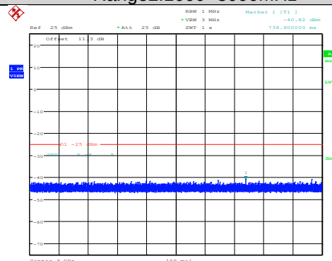
Band7-20MHz-64QAM-20850-1RB#0-Range2:1000~3000MHz
