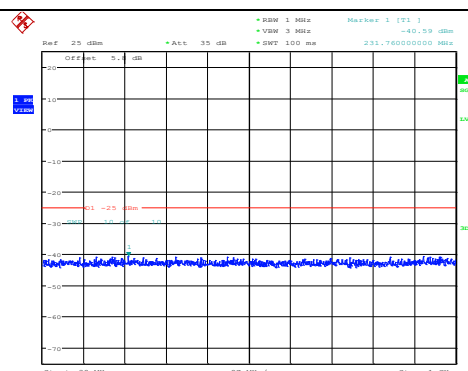
Band7-10MHz-QPSK-21400-1RB#0-Range1:30~1000MHz
