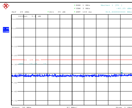
Band7-20MHz-QPSK-21100-1RB#0- Range1:30~1000MHz
