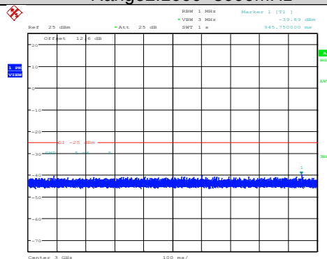
Band7-10MHz-16QAM-21100-1RB#0- Range2:1000~3000MHz
