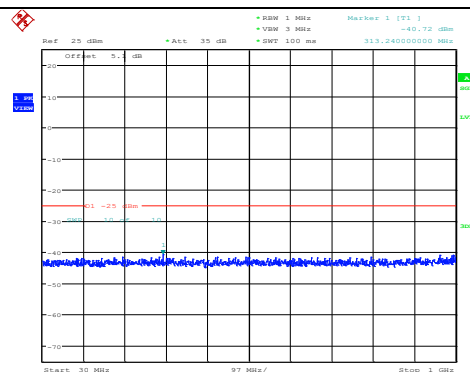
Band7-20MHz-64QAM-20850-1RB#0-Range1:30~1000MHz
