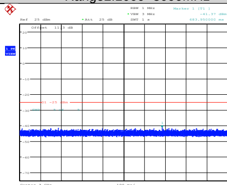
Band7-5MHz-64QAM-21425-1RB#0- Range2:1000~3000MHz
