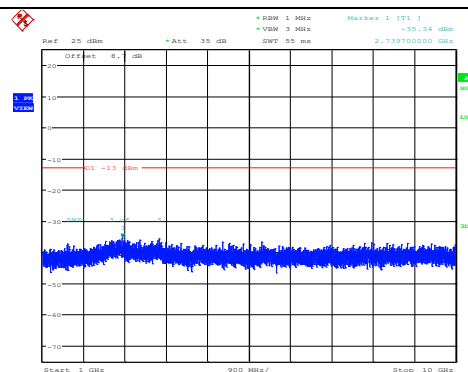
Band5-10MHz-64QAM-20525-1RB#0- Range2:1000~10000MHz
