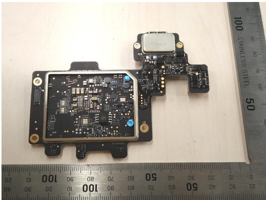
Figure 8: Mainboard view -4
