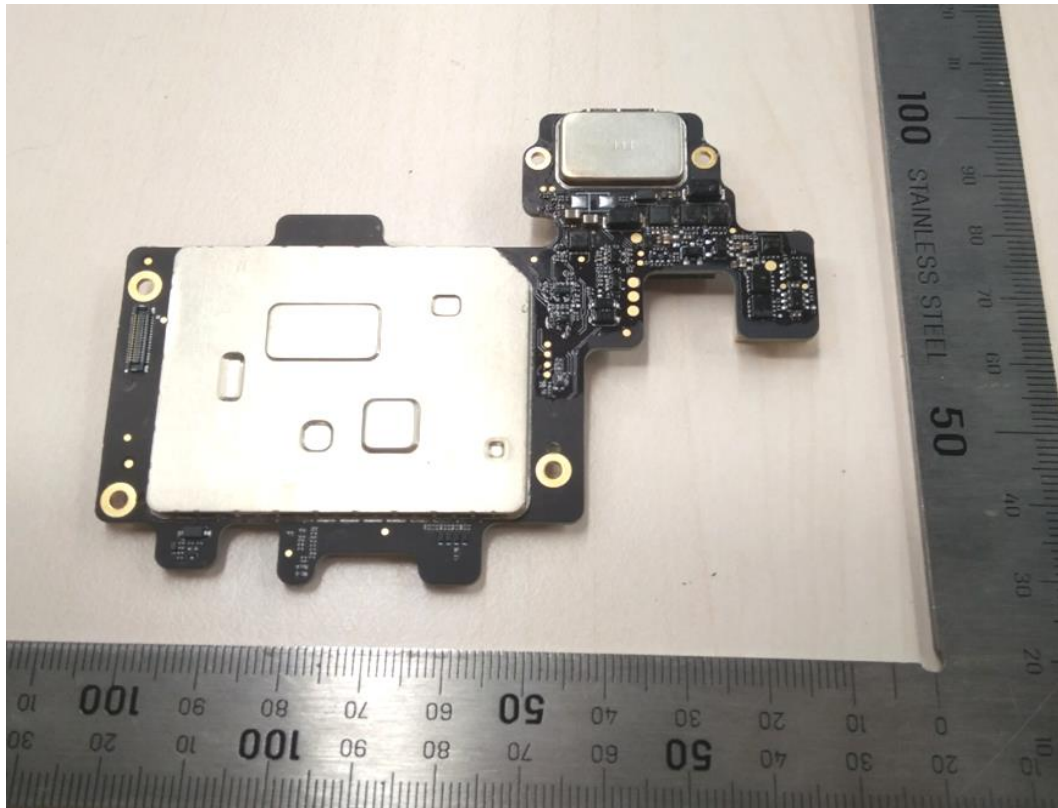
Figure 7: Mainboard view -3
