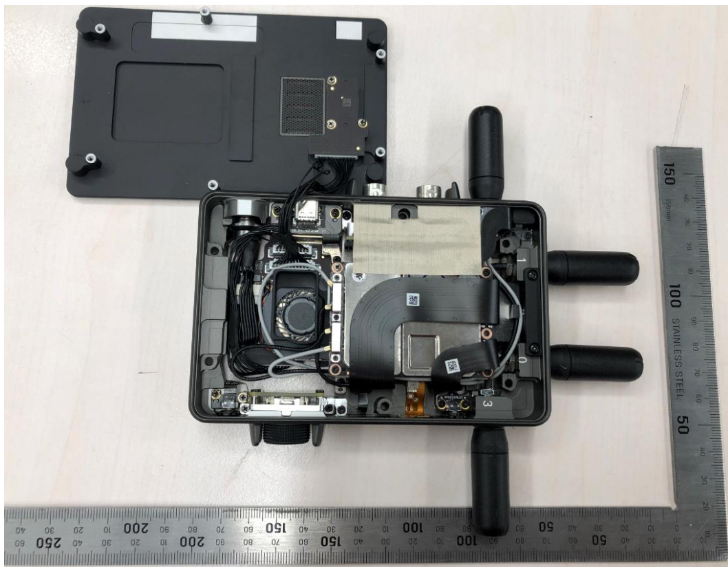
Figure 2: Internal view -2
