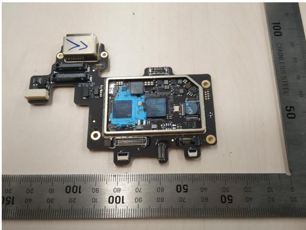
Figure 6: Mainboard view -2
