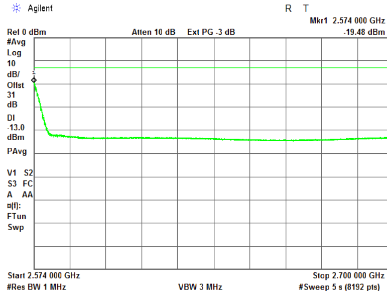
Plot 7.12.15 Spurious emission measurements in 2574 - 2700 MHz at high carrier frequency
