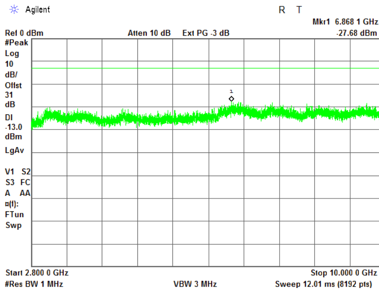
Plot 7.11.21 Spurious emission measurements in 2800 - 10000 MHz at high carrier frequency
