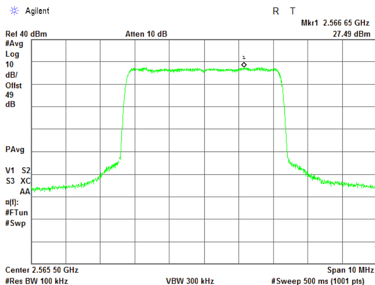
Plot 7.5.4 Power spectral density test results at low frequency, QPSK, 5 MHz EBW, RF # 2
