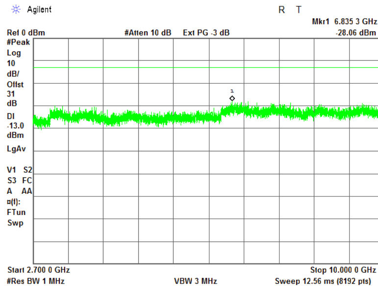
Plot 7.12.16 Spurious emission measurements in 2700-10000 MHz range at low carrier frequency
