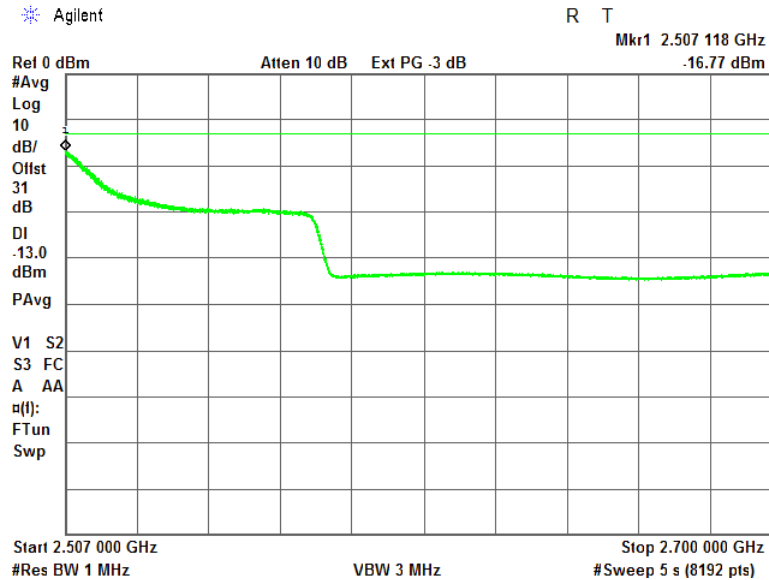
Plot 7.12.13 Spurious emission measurements in 2507 - 2700 MHz range at low carrier frequency
