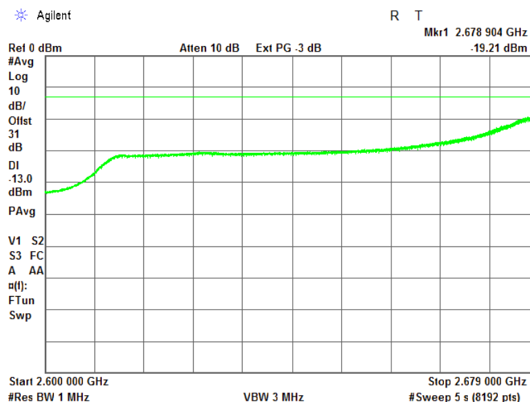
Plot 7.11.15 Spurious emission measurements in 2600 -2679 MHz at high carrier
