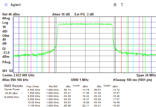
Plot 7.8.8 Spurious emission at band edges test results at mid carrier frequency, 10 MHz EBW
