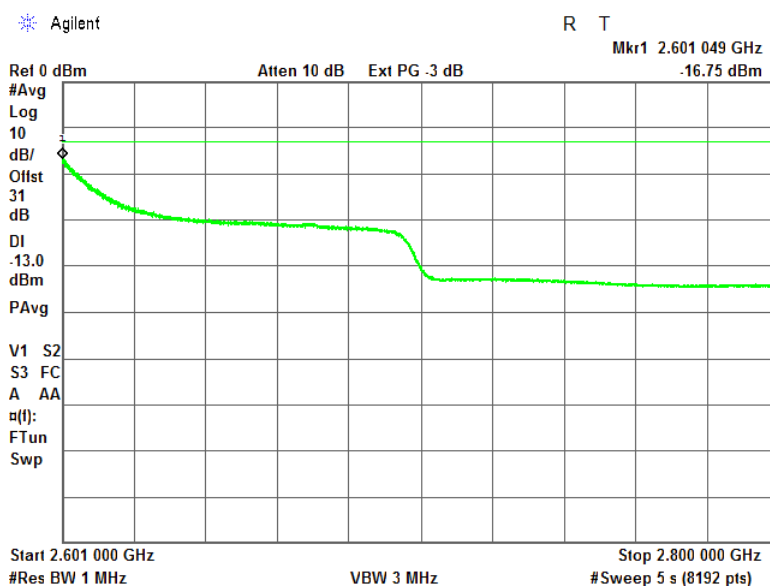
Plot 7.10.17 Spurious emission measurements in 2601 - 2800 MHz at mid carrier frequency
