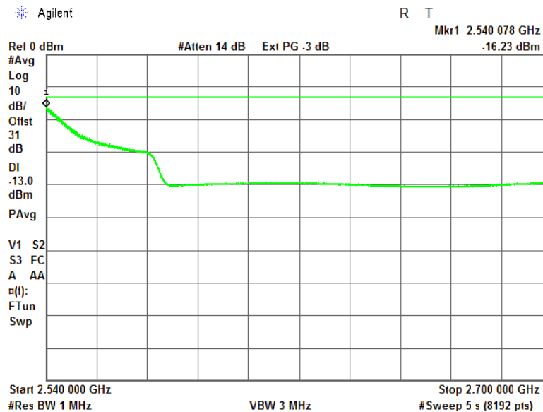
Plot 7.12.14 Spurious emission measurements in 2540 - 2700 MHz at mid carrier frequency
