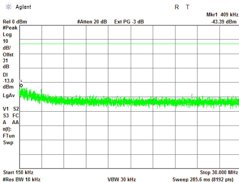
Plot 7.10.5 Spurious emission measurements in 0.15 - 30.0 MHz range at mid carrier frequency
