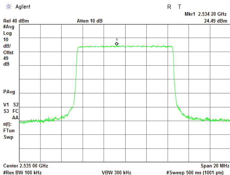
Plot 7.5.18 Power spectral density test results at high frequency, QPSK, 10 MHz EBW, RF # 2
