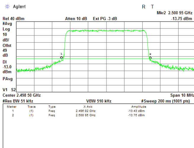
Plot 7.7.2 Spurious emission at band edges test results at mid carrier frequency, 5 MHz EBW
