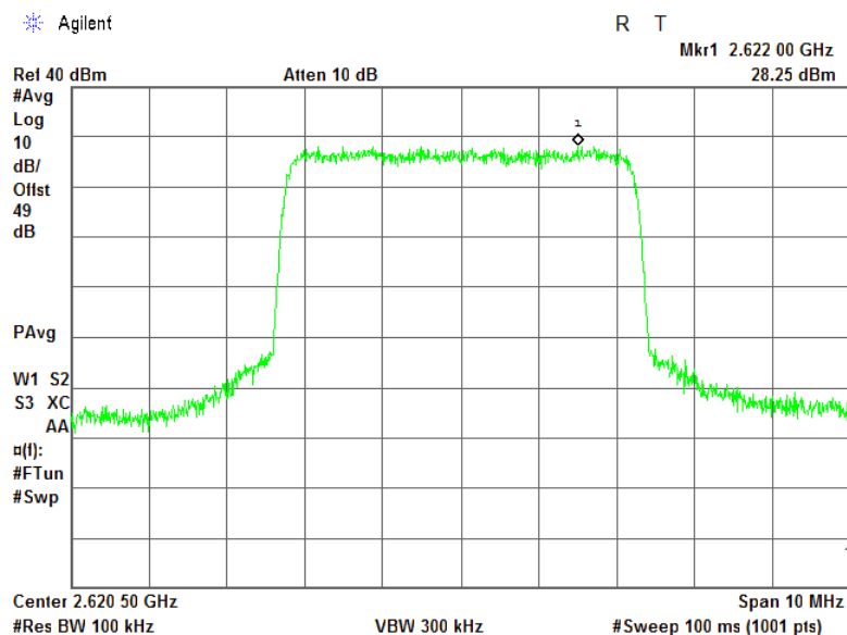
Plot 7.6.1 Power spectral density test results at low frequency, QPSK, 5 MHz EBW, RF # 1
