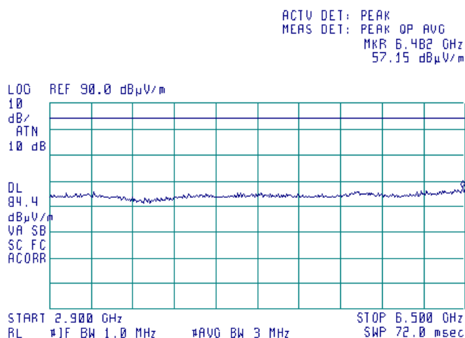
Plot 7.13.10 Radiated emission measurements in 2900 - 6500 MHz range
