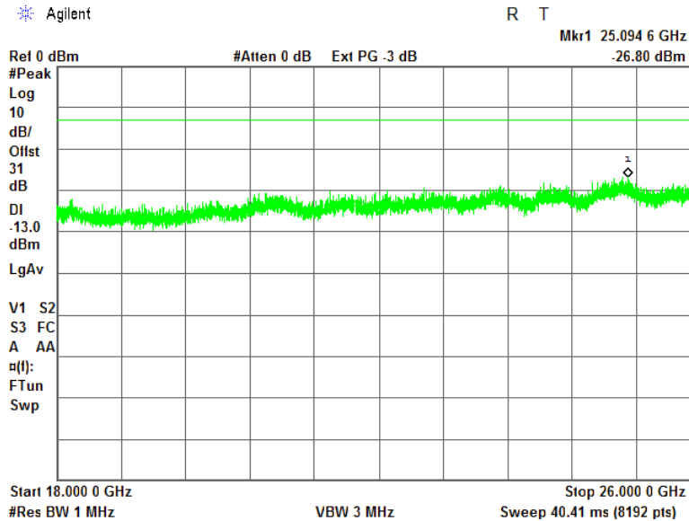
Plot 7.12.24 Spurious emission measurements in 18000 - 26000 MHz at high carrier frequency
