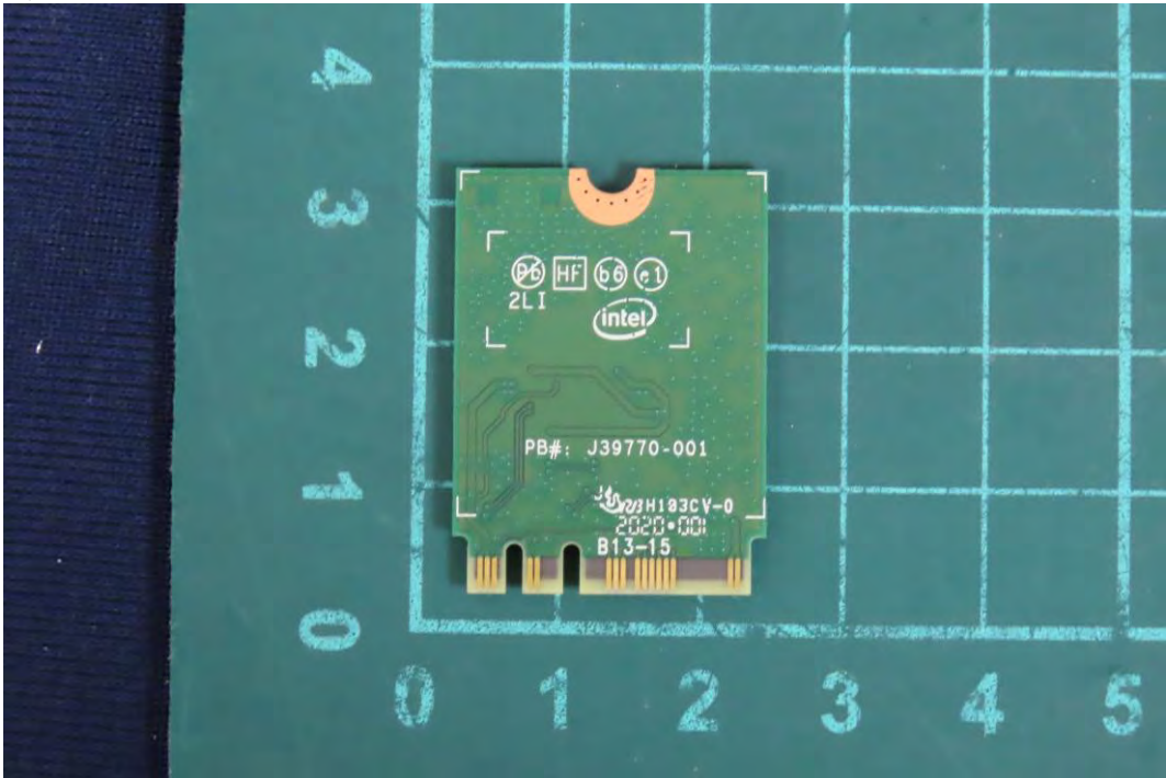
(25) EUT Photo
