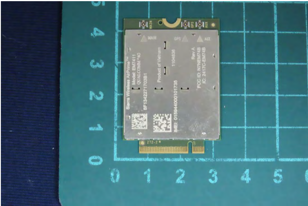
(26) EUT Photo
