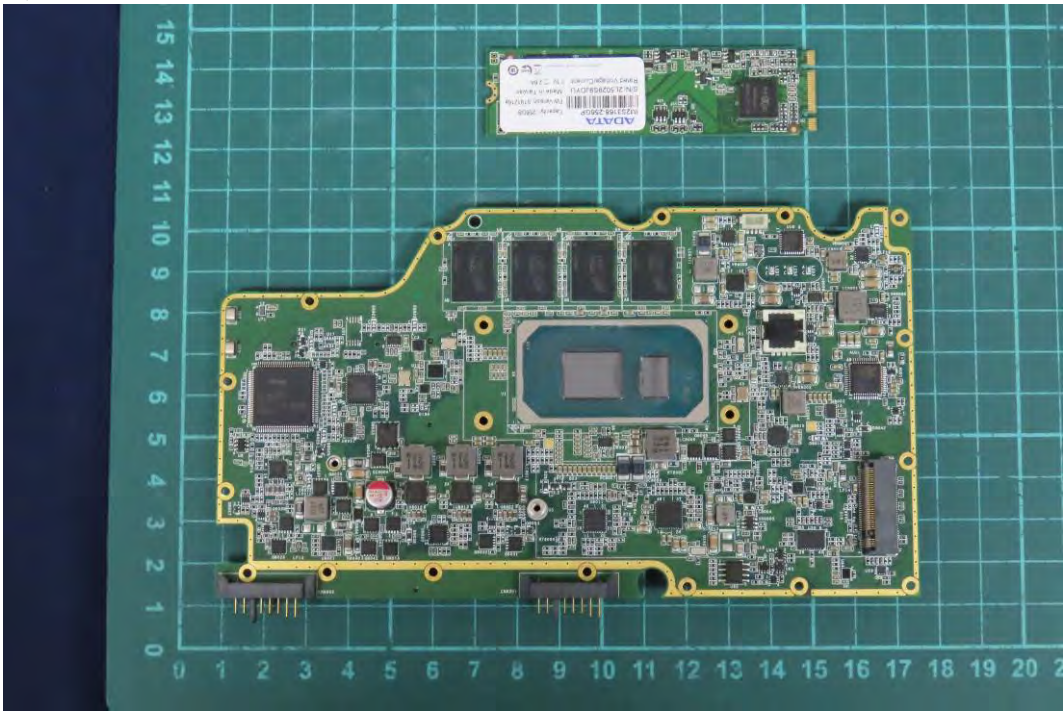
(32) EUT Photo
