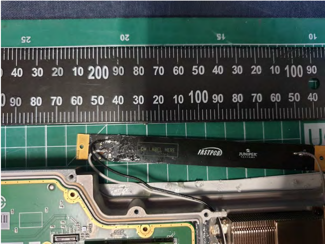
(36) EUT Photo (WiFi/BT, GPS Aux Antenna)
