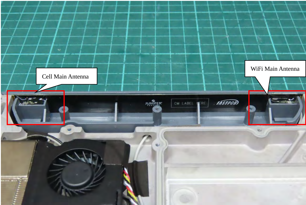
(39) EUT Photo (Main Antenna)
