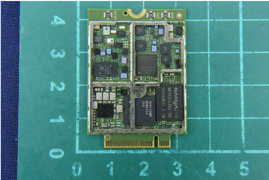
(28) EUT Photo
