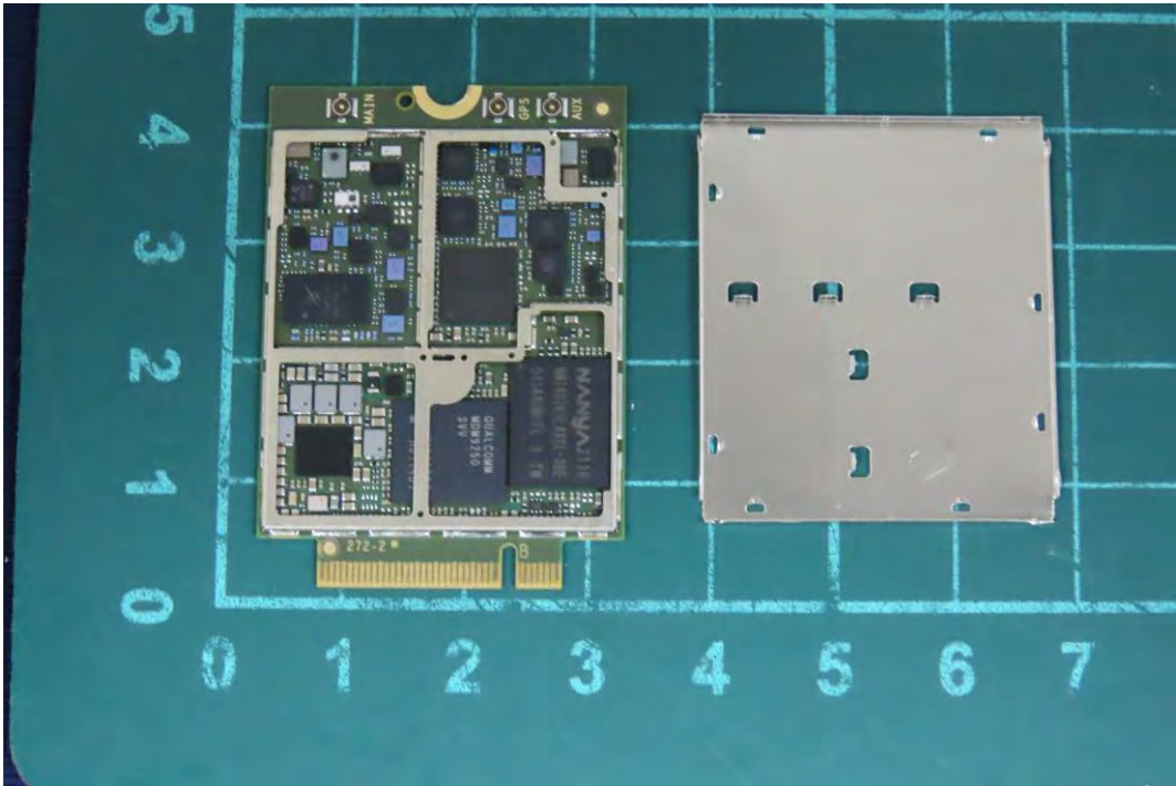
(27) EUT Photo
