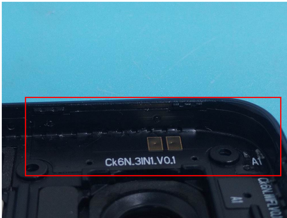
BT/2.4G Wi-Fi ANT 1
