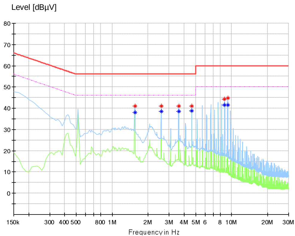
Figure 6: Spectral Diagrams, Conducted Emission, 150 kHz – 30 MHz, N, modes 1+3, power supply ICPSW24-7-3
