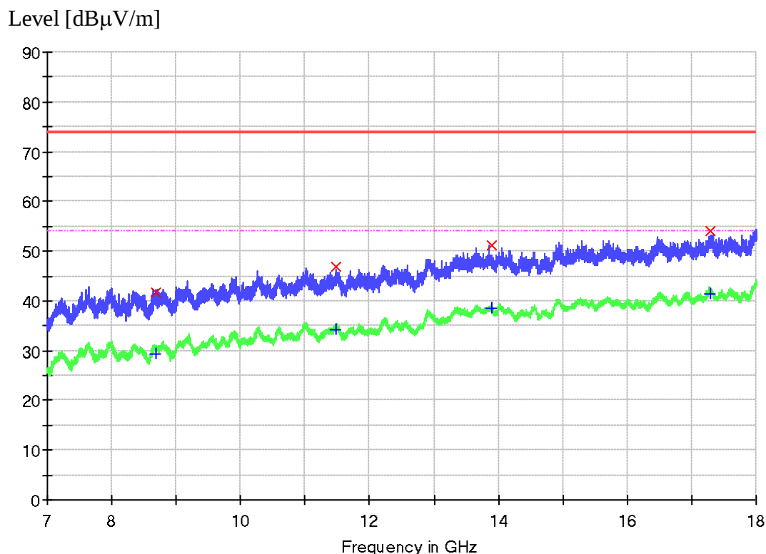
Figure 23: Spectral Diagrams and measurement results, 7-18 GHz, horizontal polarization, mode 1, power supply ICPSW24-19-1
