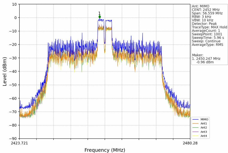
802.11ax(HEW40)_HCH_2452MHz_RU52_Mid_MIMO_NTNV
