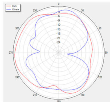
Phi=90 freq=2400MHz
