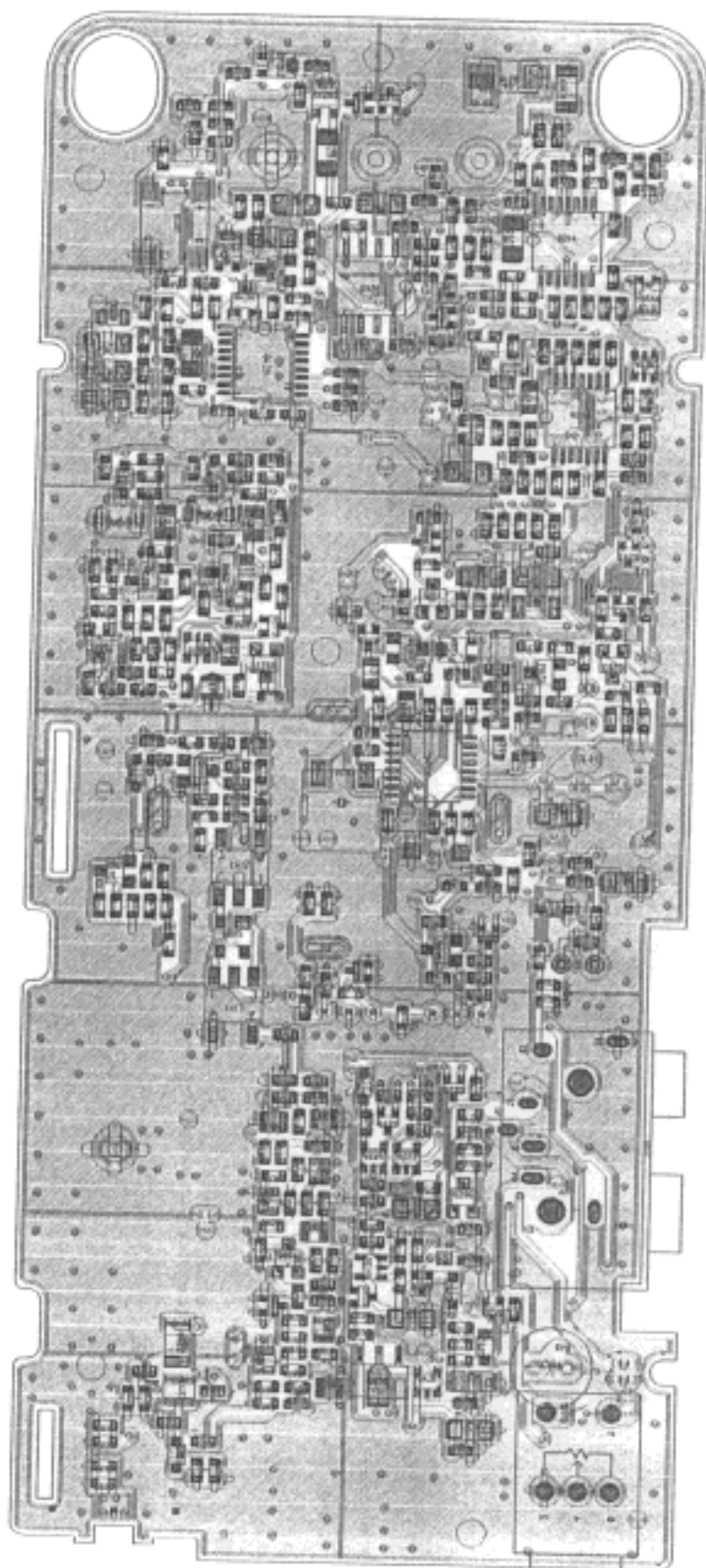
0215 Platen... Bottom View, TS-440
