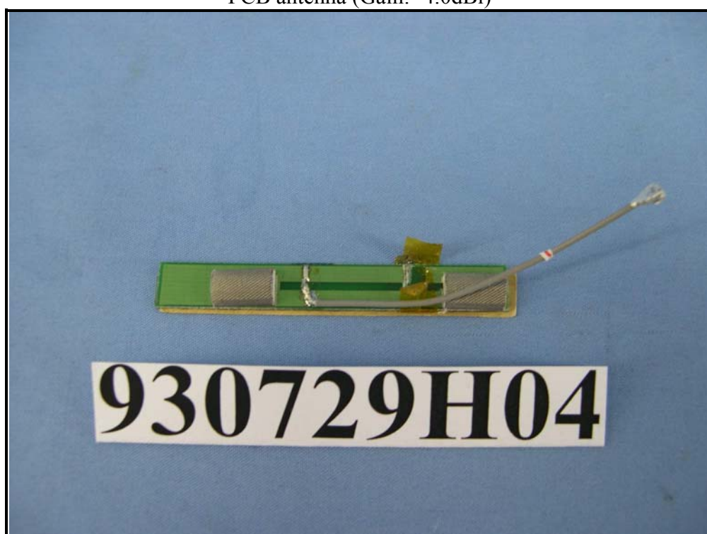
PCB antenna (Gain: -4.0dBi)
