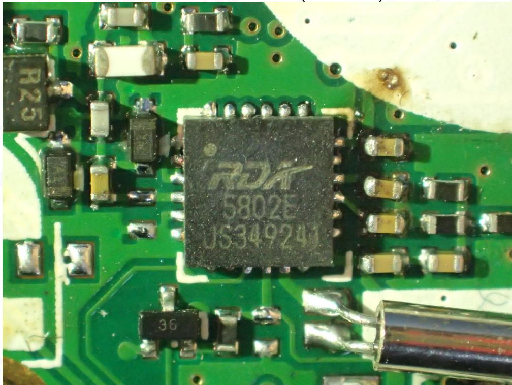
TH-UVF8 TOP VIEW OF EUT
