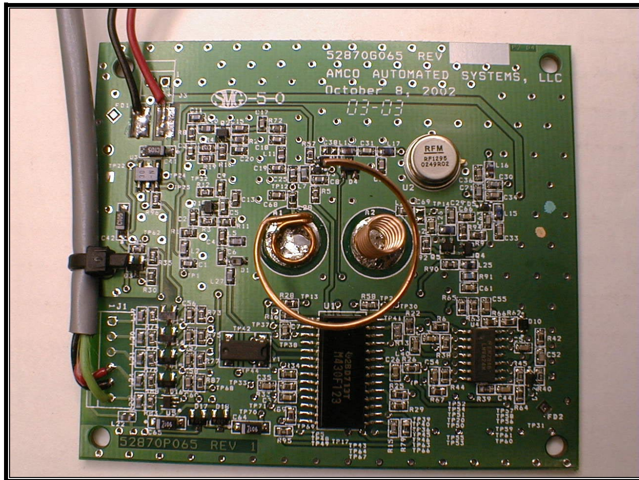
PHOTOGRAPH 7: FRONT VIEW OF BOARD
