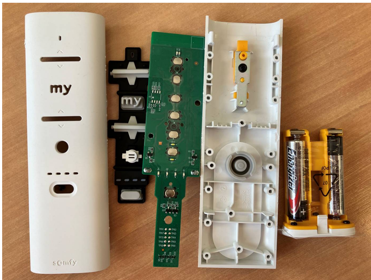
EUT- Inside View
