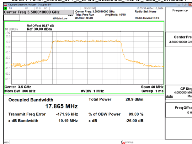
Band77-Part27_20MHz_DFT_s_OFDM_SCS30kHz_16QAM_RB50_0_CH633334
