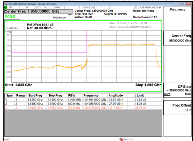
Band2_15MHz_DFT_s_OFDM_SCS15kHz_BPSK_RB75_0_CH371500
