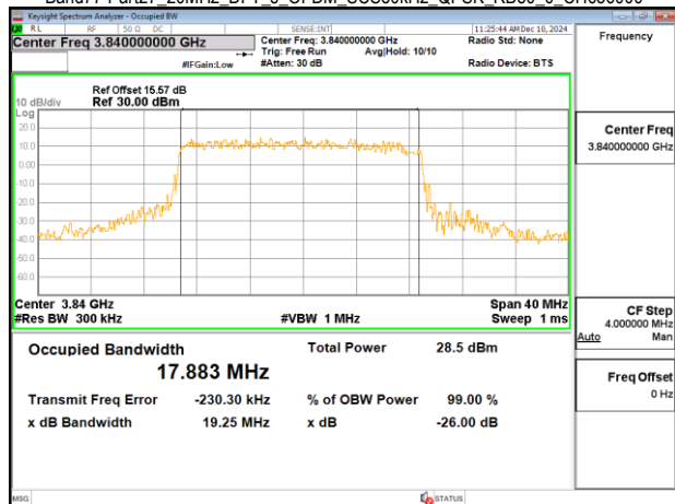
Band77-Part27_20MHz_DFT_s_OFDM_SCS30kHz_QPSK_RB50_0_CH656000
