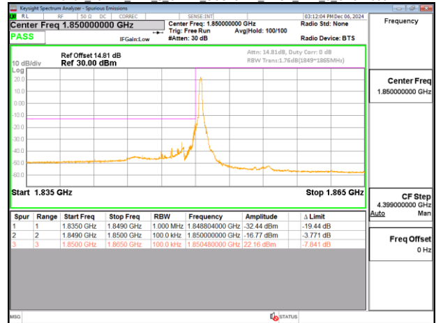
Band2_15MHz_DFT_s_OFDM_SCS15kHz_BPSK_RB75_0_CH371500
