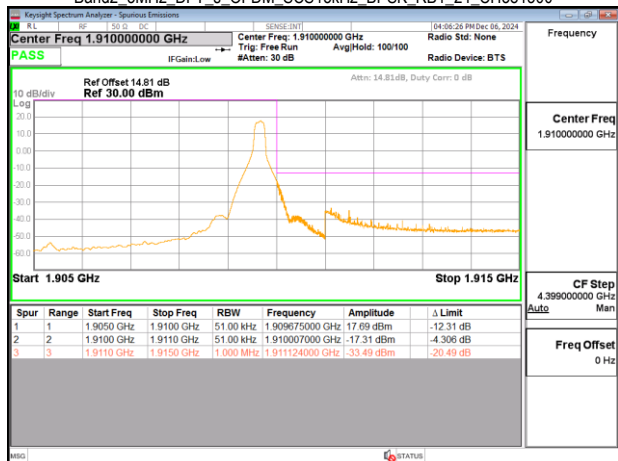
Band2_5MHz_DFT_s_OFDM_SCS15kHz_BPSK_RB1_24_CH381500
