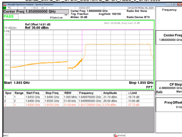
Band2_5MHz_CP_OFDM_SCS15kHz_QPSK_RB25_0_CH370500
