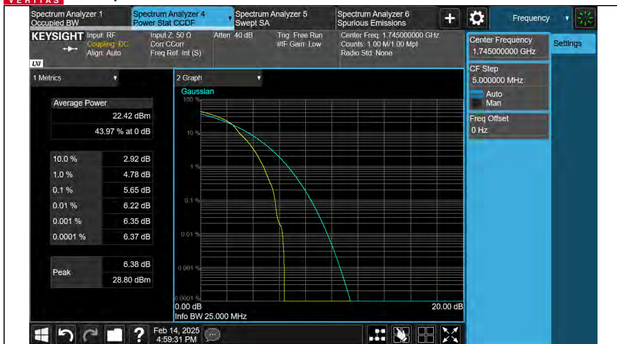
Band66-20MHz-16QAM-132322-27RB#0
