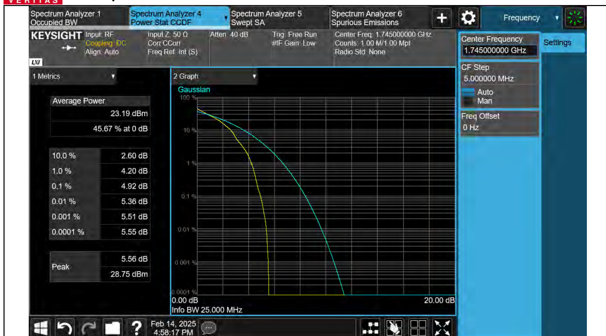
Band66-20MHz-QPSK-132322-100RB#0
