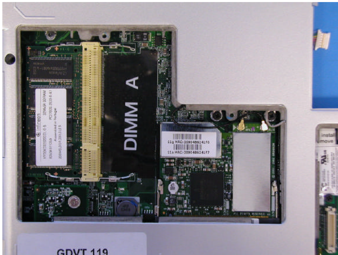
Ram and Wireless access
