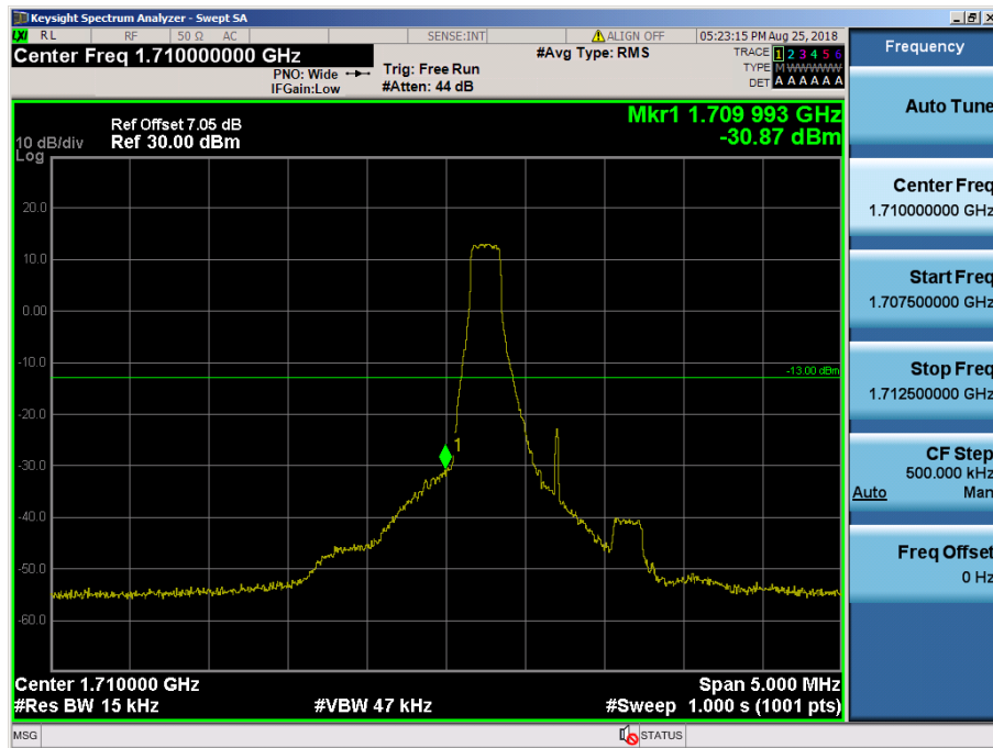
LTE Band 4 / 1.4MHz / 64QAM - RB Size/Offset (1/0)
