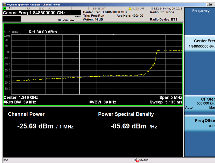
LTE Band 2 / 5MHz / 64QAM Offset/Size (12/0)
