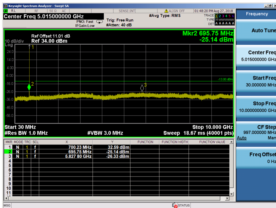
LTE Band 12 / 1.4MHz / 64QAM - RB Size/Offset (3/2) – Low Channel
