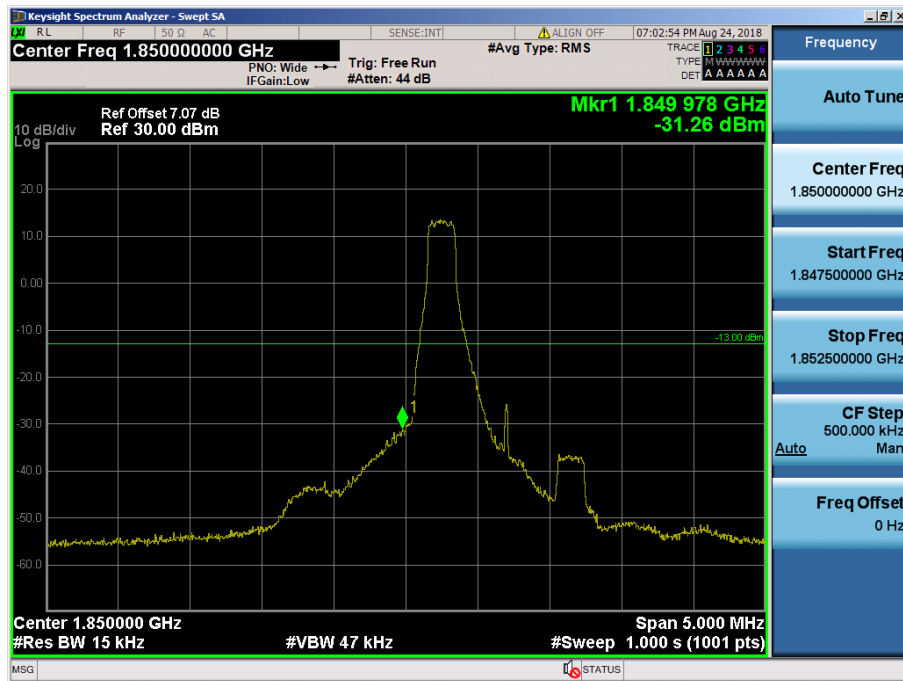
LTE Band 2 / 1.4MHz / 64QAM - RB Size/Offset (1/0)
