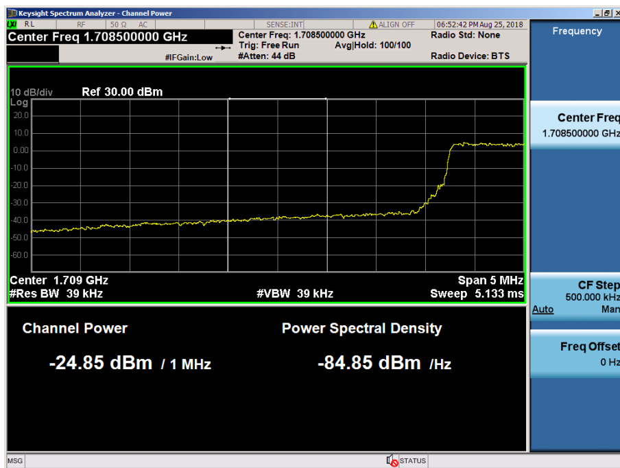
LTE Band 4 / 5MHz / 64QAM Offset/Size (12/0)
