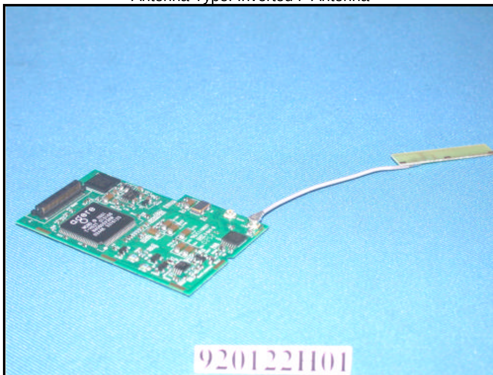
Antenna Type: Inverted F Antenna
