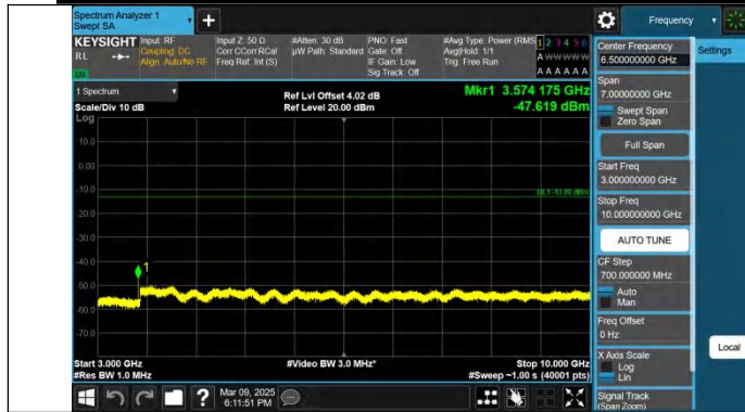
Band12-1.4MHz-QPSK-23173-1RB#0-3000~10000-PASS
