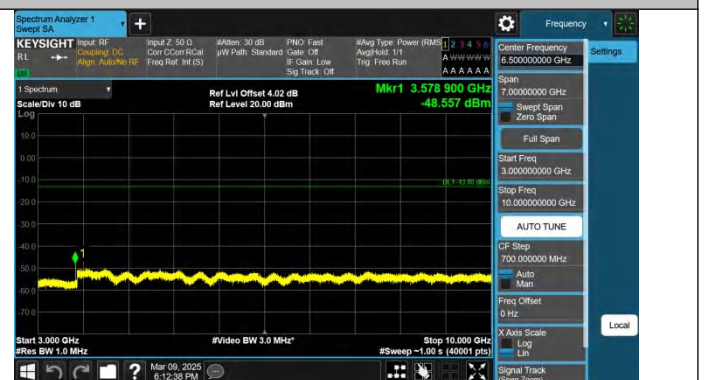
Band12-1.4MHz-QPSK-23173-1RB#5-3000~10000-PASS
