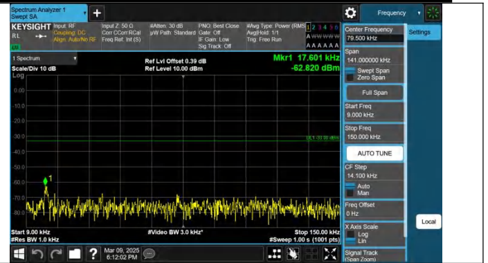
Band12-1.4MHz-QPSK-23173-1RB#5-0.009~0.15-PASS
