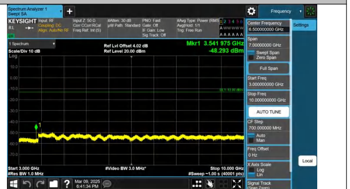
Band12-10MHz-QPSK-23060-1RB#49-3000~10000-PASS
