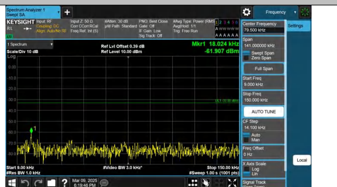
Band12-3MHz-QPSK-23025-1RB#14-0.009~0.15-PASS
