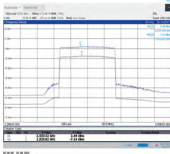
1-N41--30-100-L-2-CP-256QAM-Outer_Full-273@0- Ant1-9.63-100%-0.00-9.63-PASS-≤13
