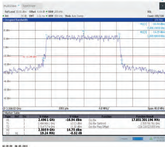
1-N41--30-20-L-3-DFT-16QAM-Outer_Full-50@0-Ant 1-17.851-19.240≤20-PASS
