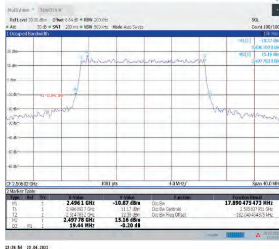
1-N41--30-20-L-4-DFT-64QAM-Outer_Full-50@0-An t1-17.89-19.440≤20-PASS
