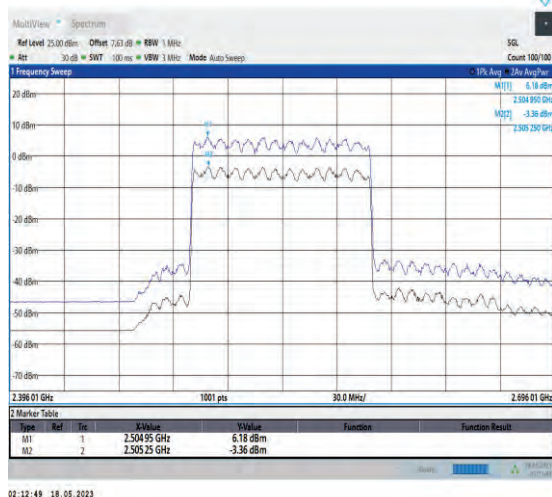
1-N41-PC1-30-100-L-1-DFT-256QAM-Outter_Full-270@0-Ant1-9.54-19.56%-7.09-2.45-PASS-≤13
