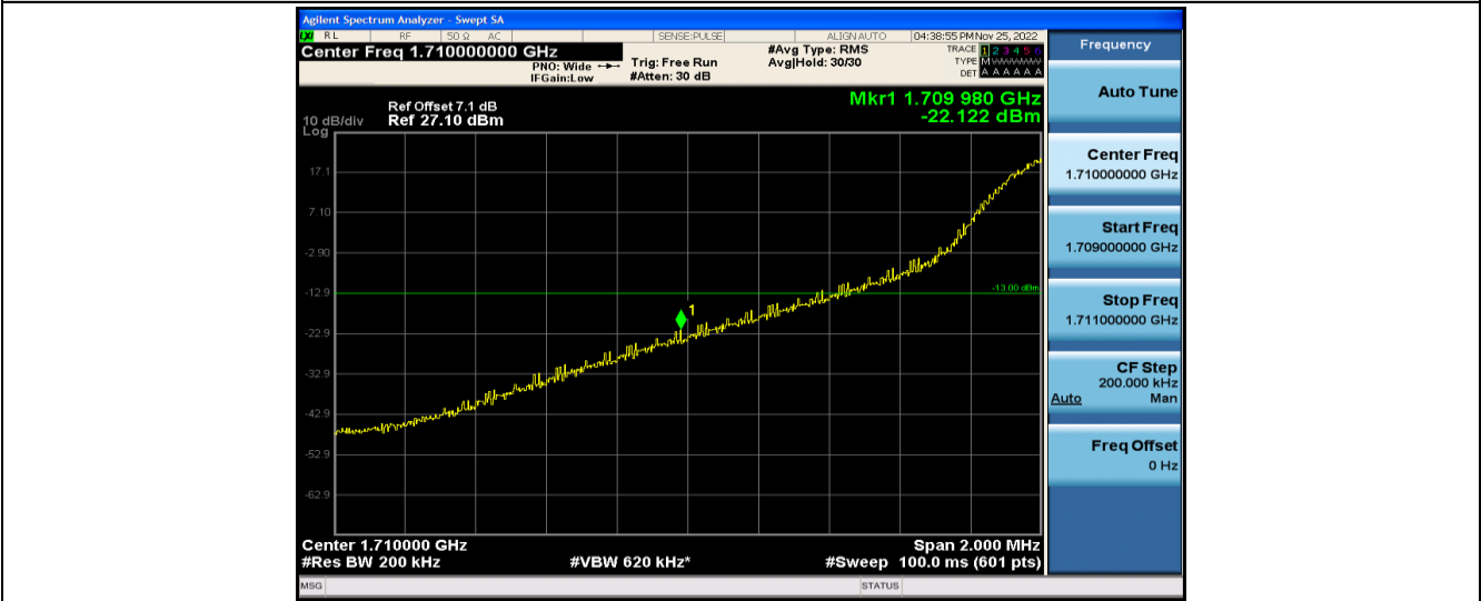
Band4-20MHz-64QAM-20050-1RB#0
