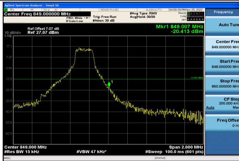
Band5-1.4MHz-64QAM-20643-1RB#5
