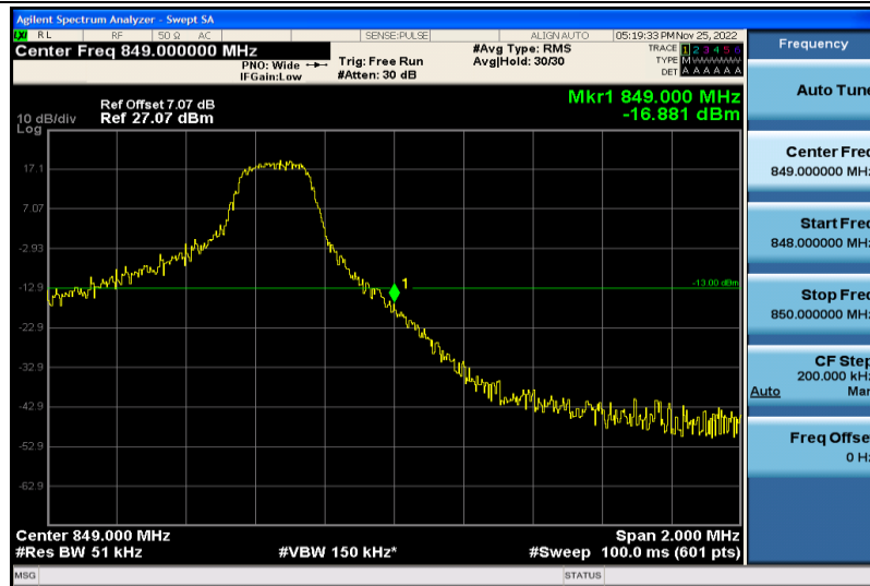
Band5-5MHz-64QAM-20625-1RB#24
