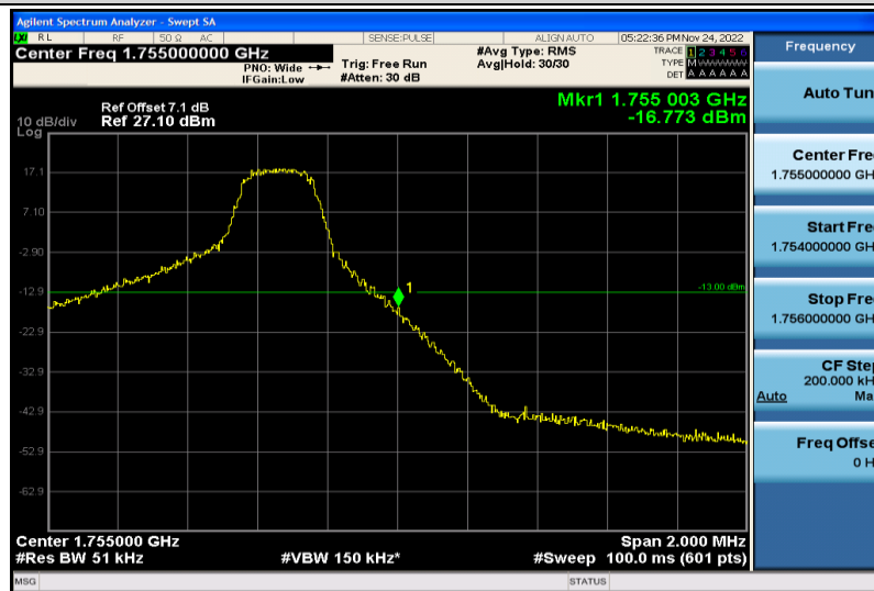
Band4-5MHz-16QAM-20375-1RB#24
