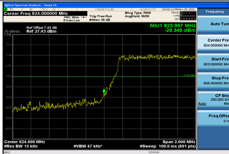
Band5-1.4MHz-64QAM-20407-6RB#0
