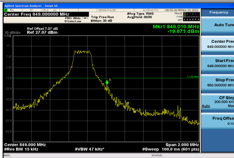
Band5-1.4MHz-16QAM-20643-1RB#5
