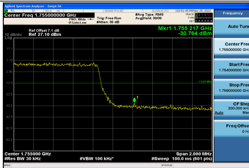
Band4-3MHz-64QAM-20385-15RB#0
