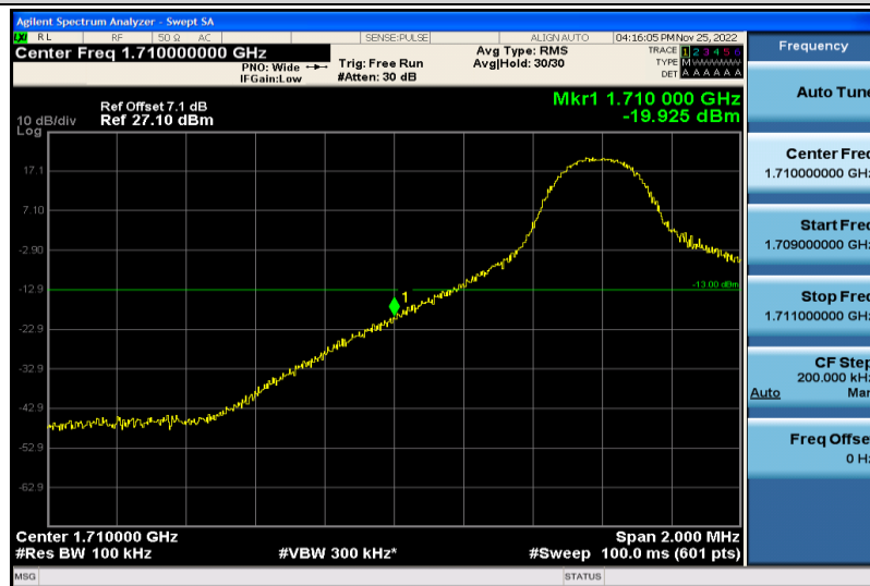
Band4-10MHz-64QAM-20000-1RB#0
