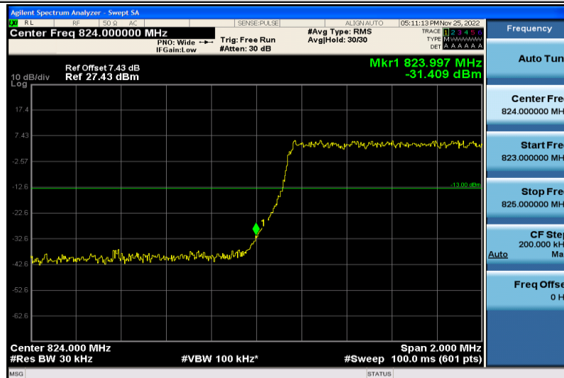
Band5-3MHz-64QAM-20415-15RB#0
