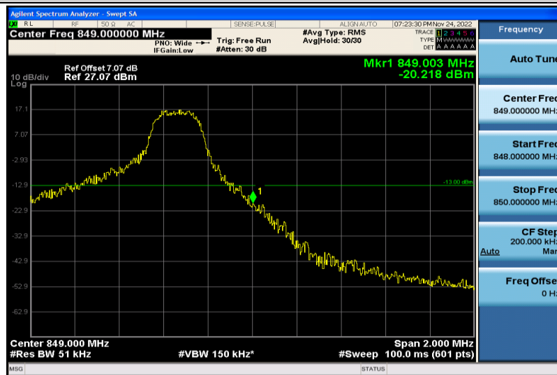
Band5-5MHz-16QAM-20625-1RB#24
