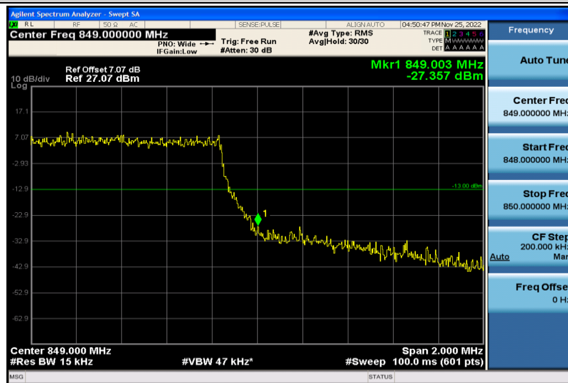
Band5-1.4MHz-64QAM-20643-6RB#0
