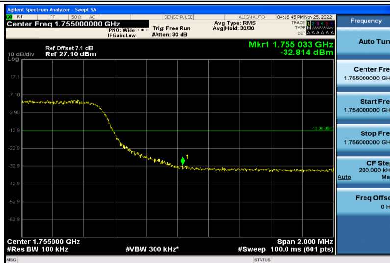
Band4-10MHz-64QAM-20350-50RB#0
