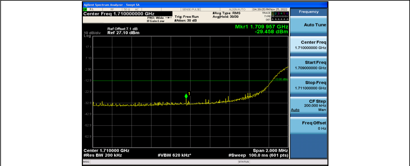
Band4-20MHz-64QAM-20050-100RB#0
