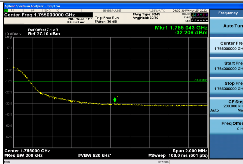
Band4-20MHz-64QAM-20300-100RB#0
