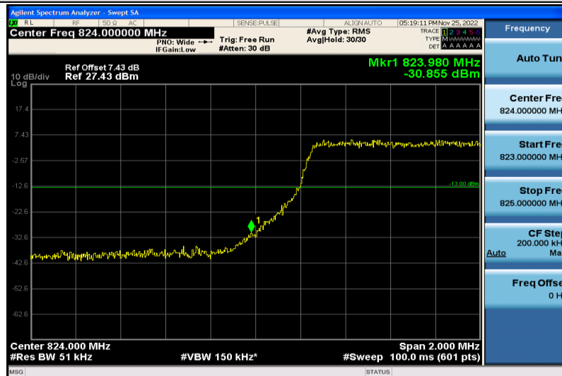
Band5-5MHz-64QAM-20425-25RB#0
