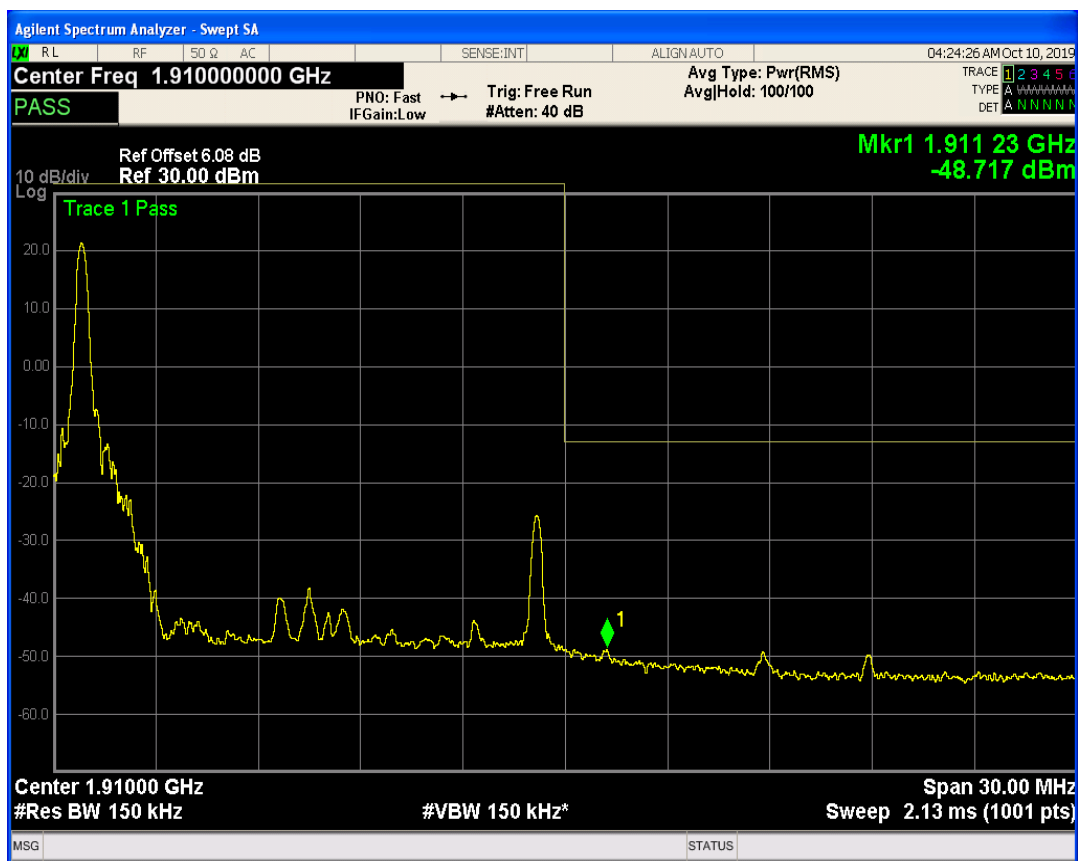
LTE Band2 QPSK BW=15MHz Channel=19125 RB Size=1 Position=#Max
