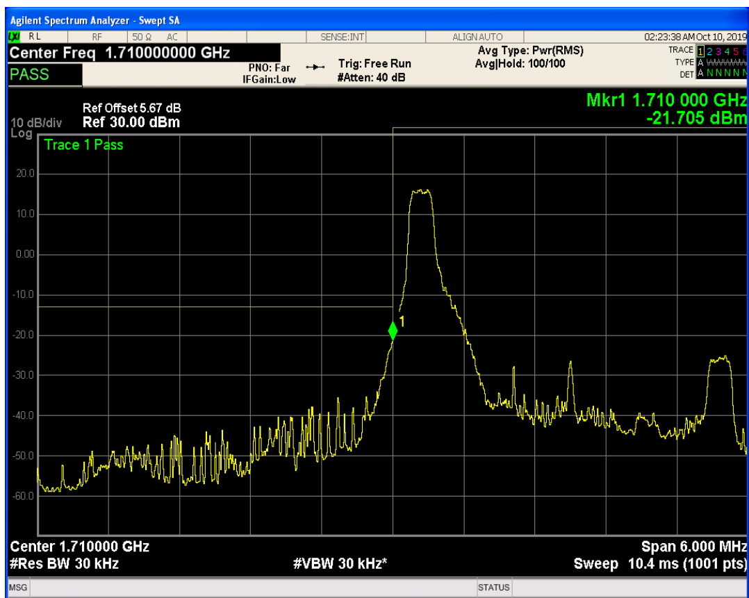
LTE Band4 QPSK BW=3MHz Channel=19965 RB Size=1 Position=#Max
